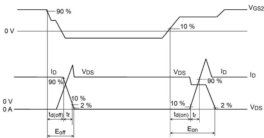
Fig. 6.5.2 Timing Diagram
