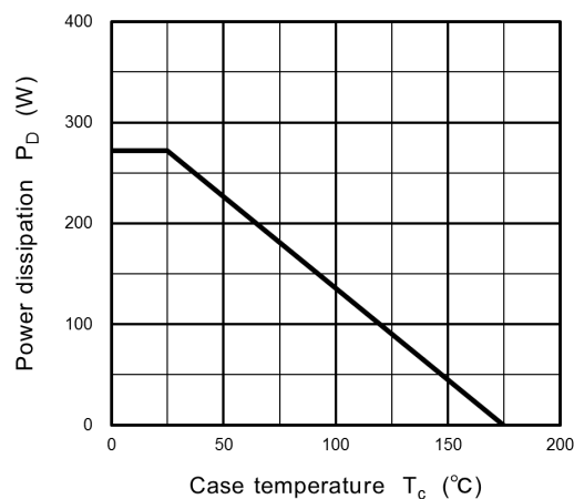
Fig. 8.13 P_D - T_c (Guaranteed Maximum)
