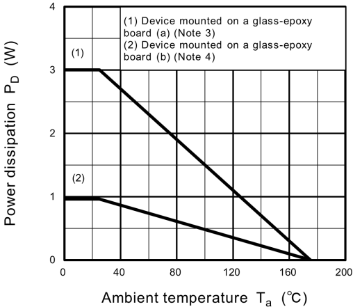
Fig. 8.15 P_D - T_a (Guaranteed Maximum)
