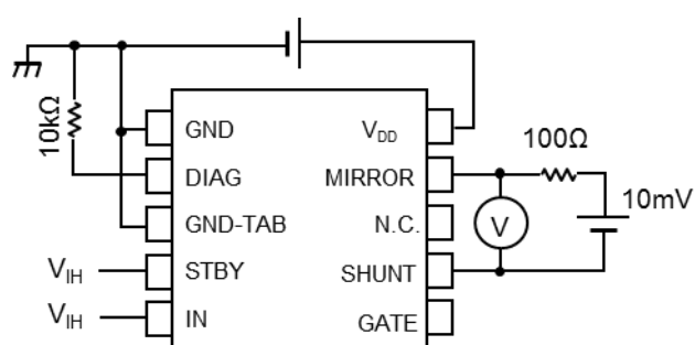
Figure 11.4 Test Circuit 4
