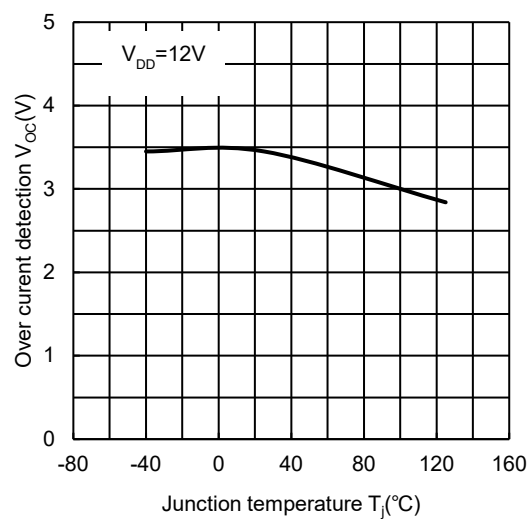
V_{OC} - T_j
