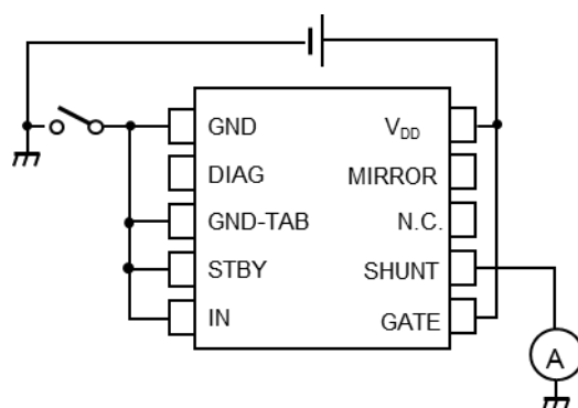
Figure 11.3 Test Circuit 3
