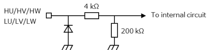
Figure 6.1 Equivalent circuit (1)
