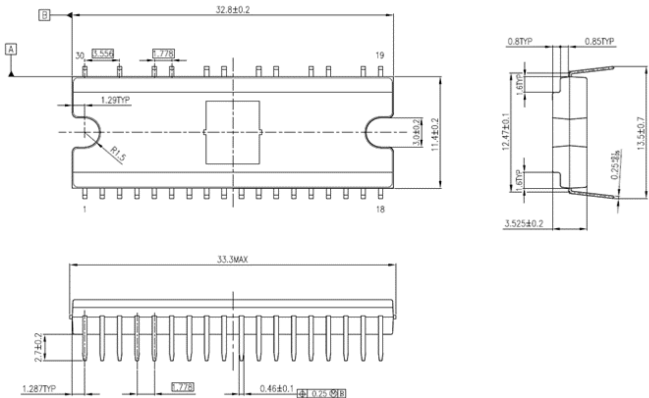
Figure 12.1 Package Dimensions
