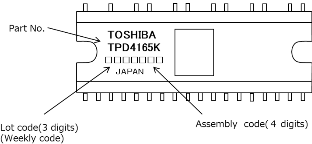
Figure 5.2 Marking
