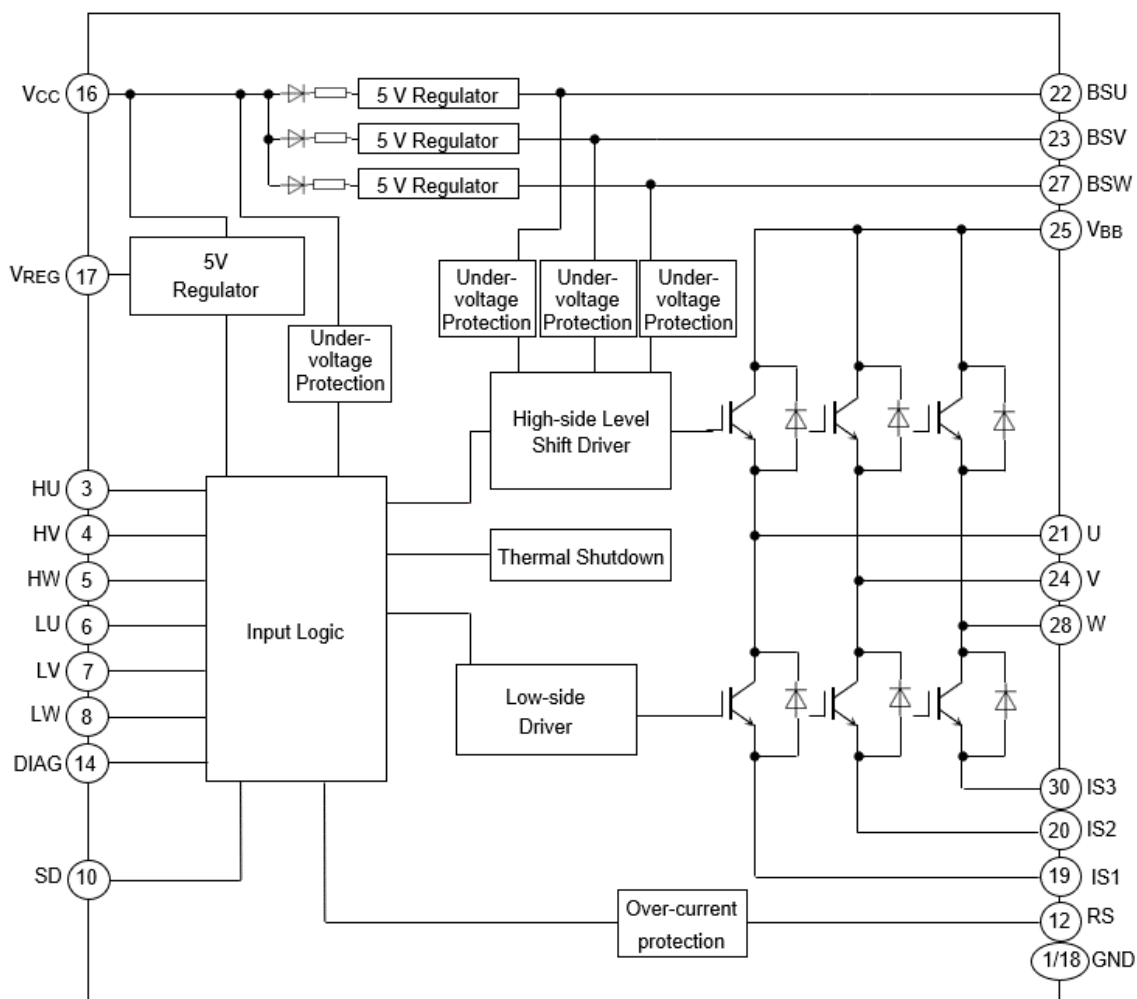
Figure 4.1 Block Diagram
