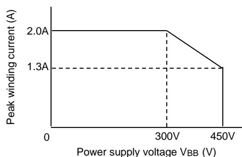
Figure10.1 SOA at T_j = 135\text{ }^{\circ}\text{C}
