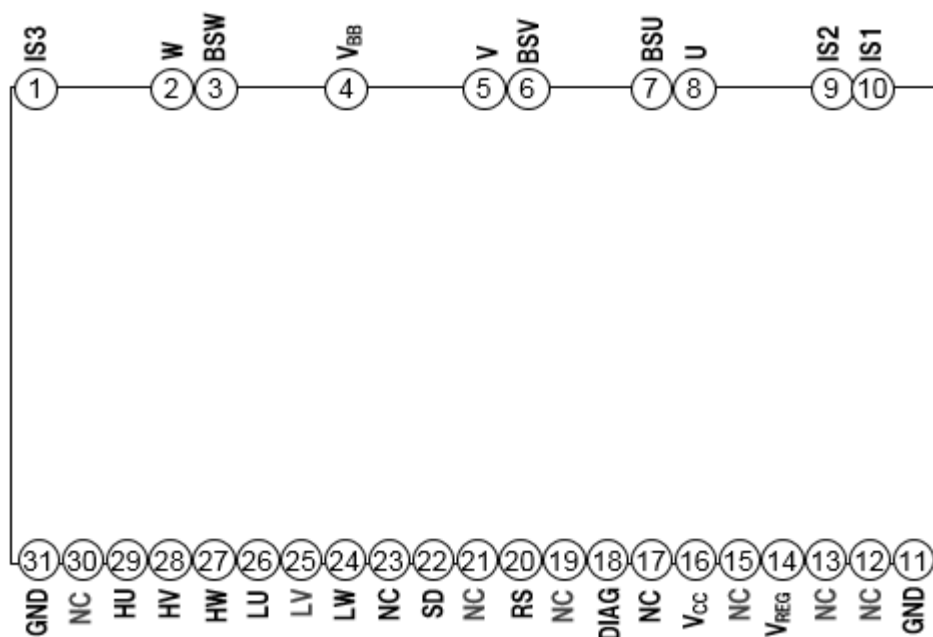
Figure 5.1 Pin Assignments
