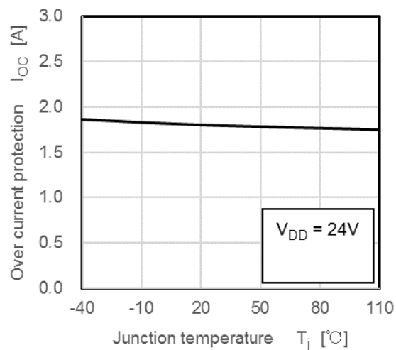
I_{OC} - T_j
