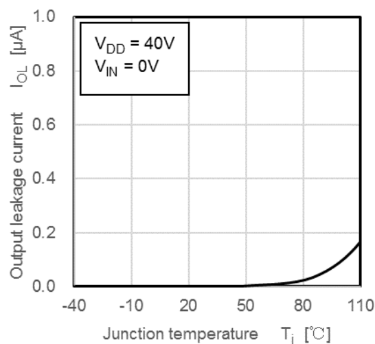
I_{OL} - T_j
