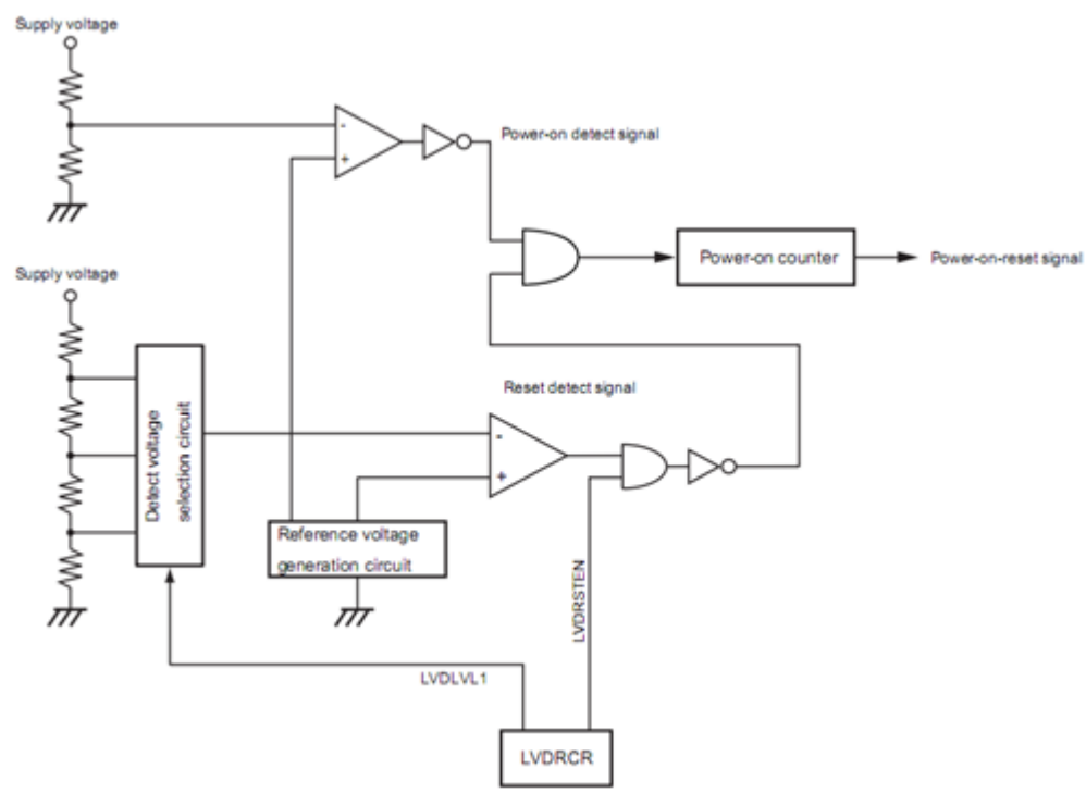
Figure 8.3 Power-on-reset circuit
