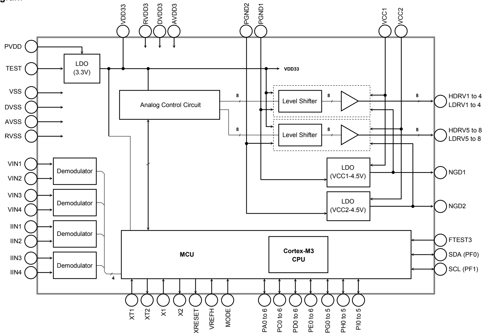
Figure 4.1 Block Diagram
