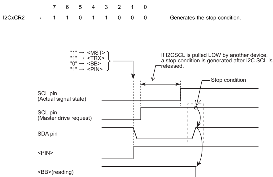
Figure 15-15 Generating the Stop Condition
