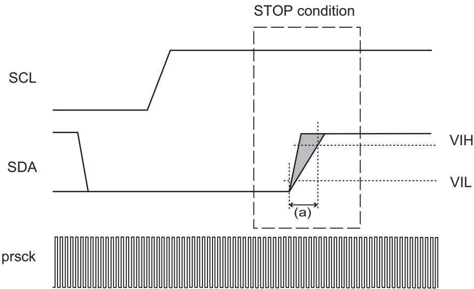
Figure 15-8 Recognition of STOP condition (condition of tr)
