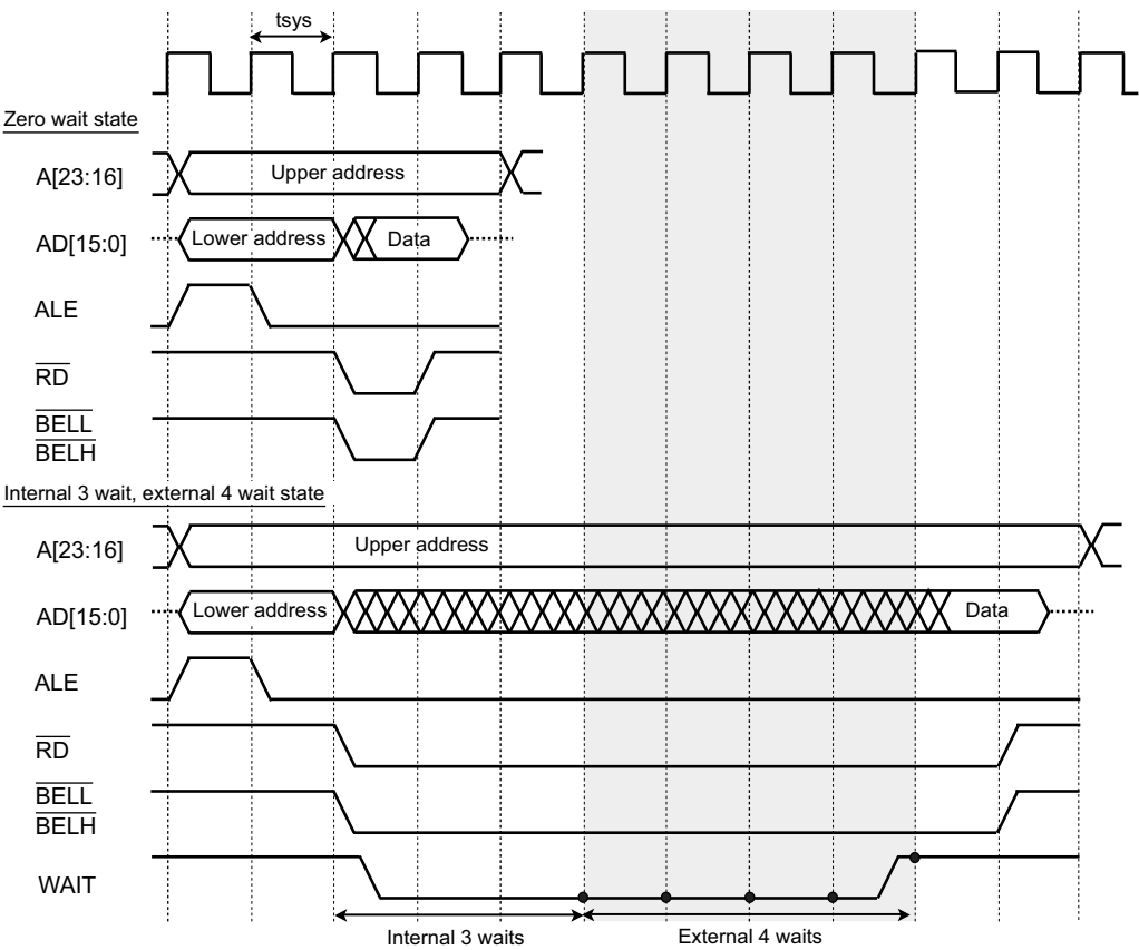
Figure 10-7 Read operation timing (External wait)
