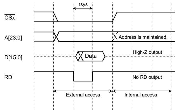
Figure 10-1 Read Operation Timing
