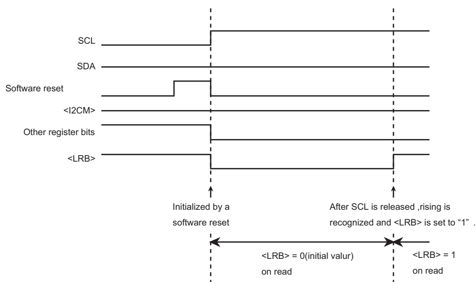
Figure 15-17 Software reset release to the SCL "LOW" to "HIGH" while SDA="HIGH"
