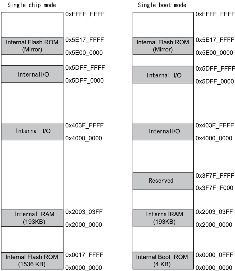
Figure 24-2 Comparison of memory map (TMPM462F15FG)
