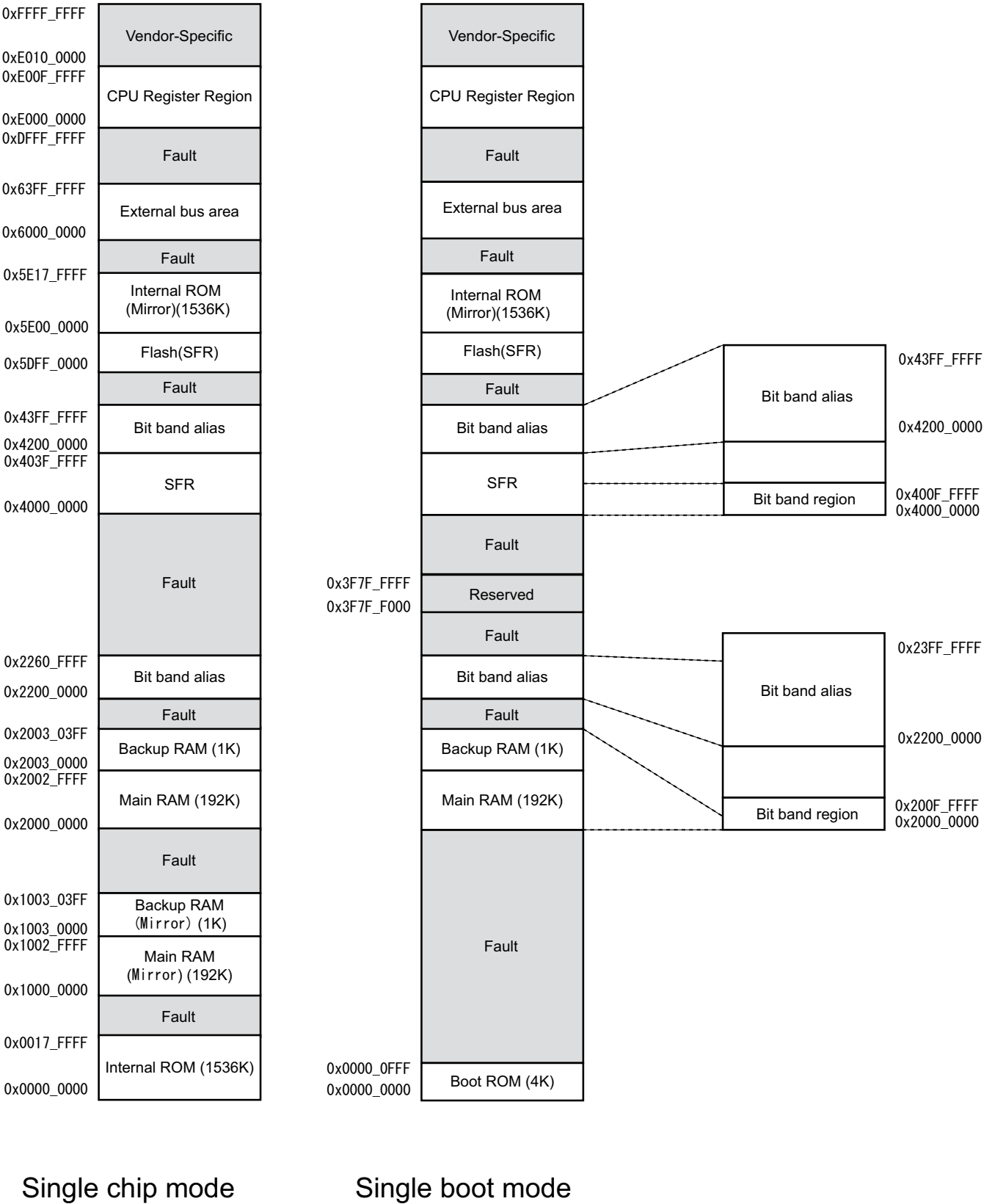
Figure 4-1 MemoryMap(1536KB)
