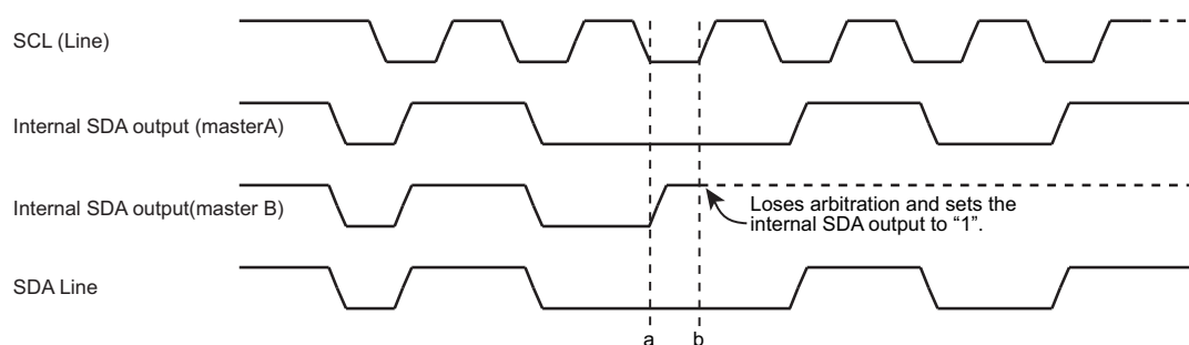
Figure 15-9 Lost Arbitration
