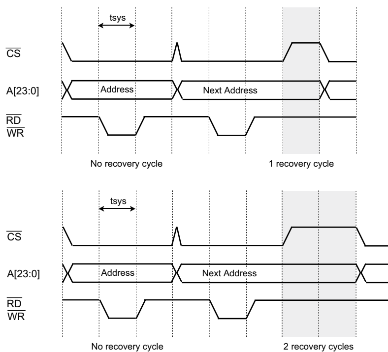
Figure 10-10 Timing of chip select recovery time insertion
