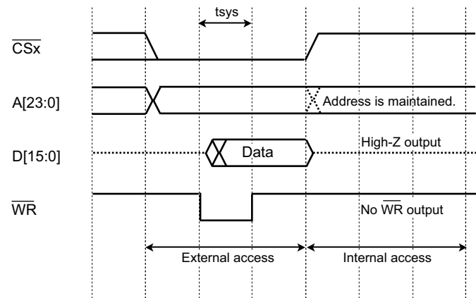
Figure 10-2 Write Operation Timing
