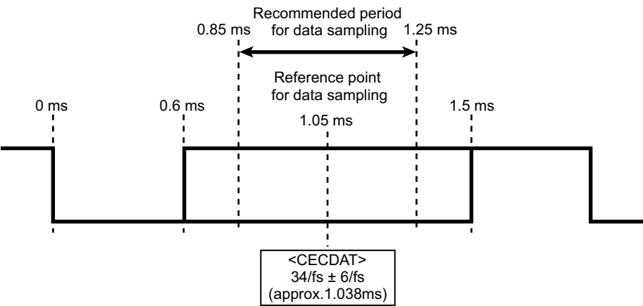
Data sampling timing that specification recommends
