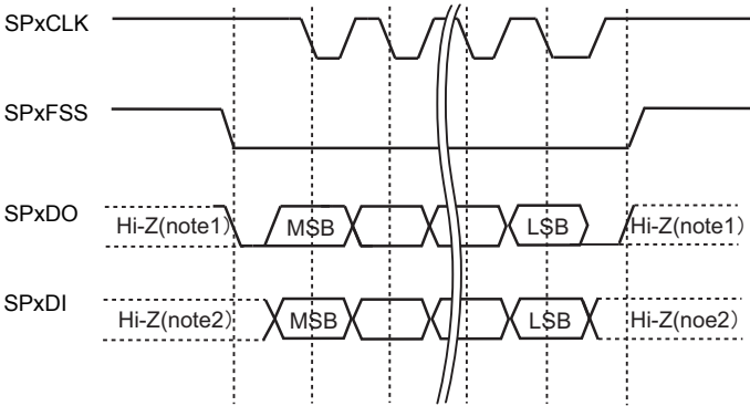
Figure 16-7 SPI frame format (single transfer, <SPO>="1" & <SPH>="0")
