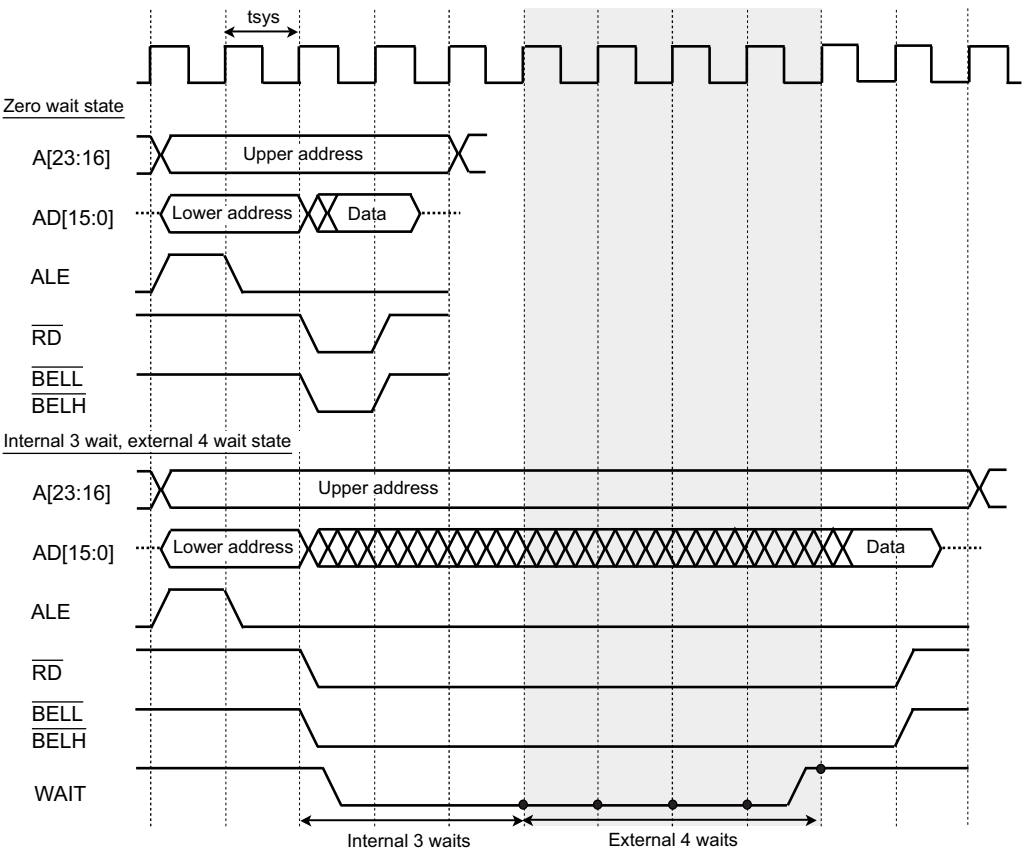
Figure 10-16 Read operation timing (External wait)
