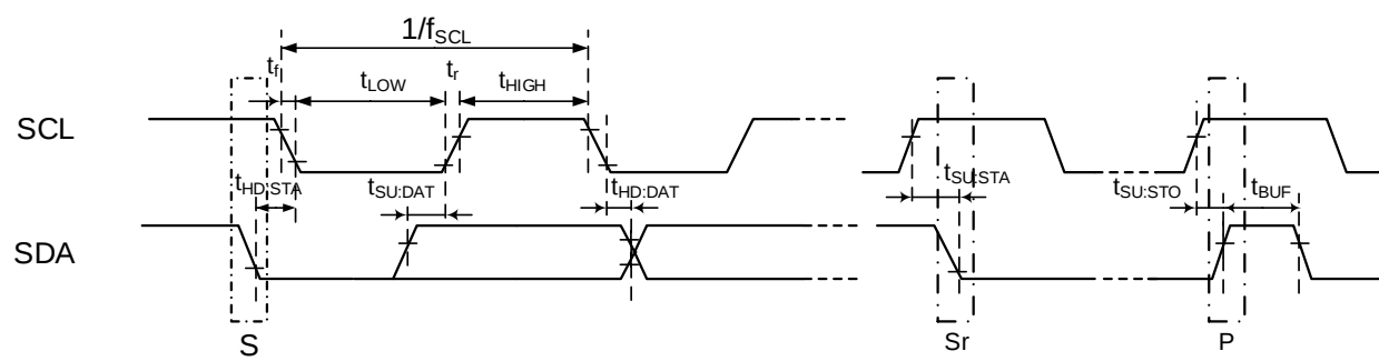
Figure 7.4 AC timing of I 2 C
