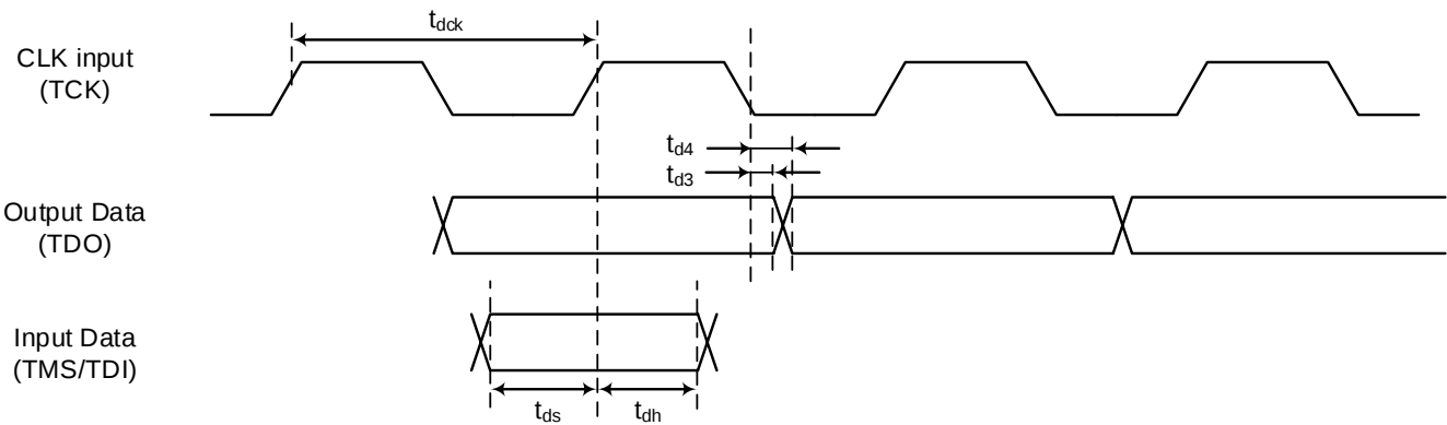
Figure 7.7 JTAG waveform
