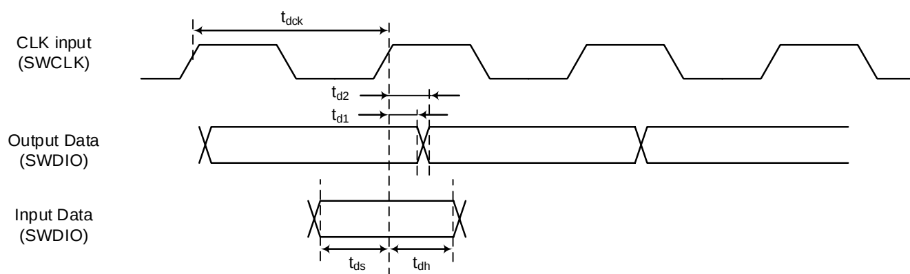
Figure 7.6 SWD waveform
