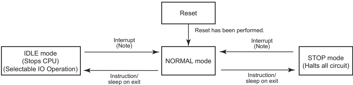
Figure 5-3 Mode Transition Diagram
