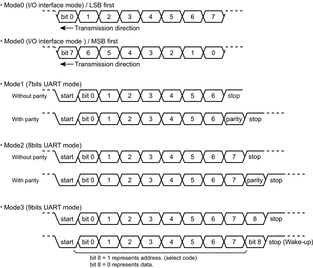
Figure 9-2 Data Format
