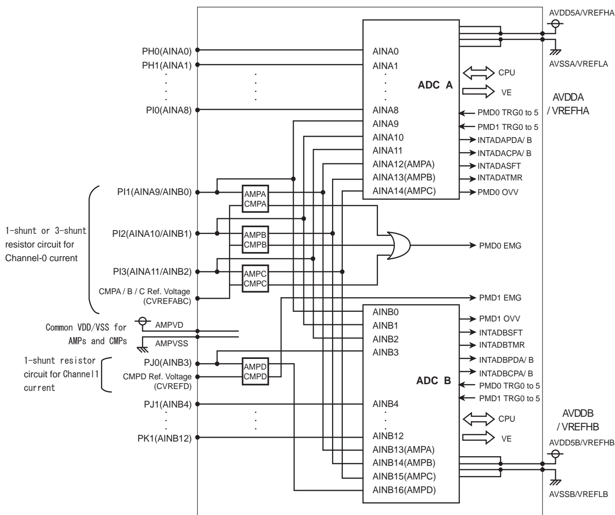
Figure 18-1 Op-Amps/Analog Converters Block Diagram
