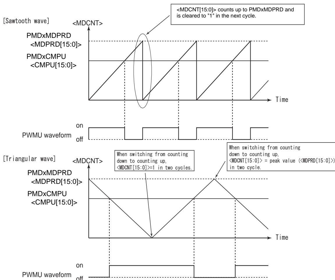
Figure 11-4 PWM Waveforms
