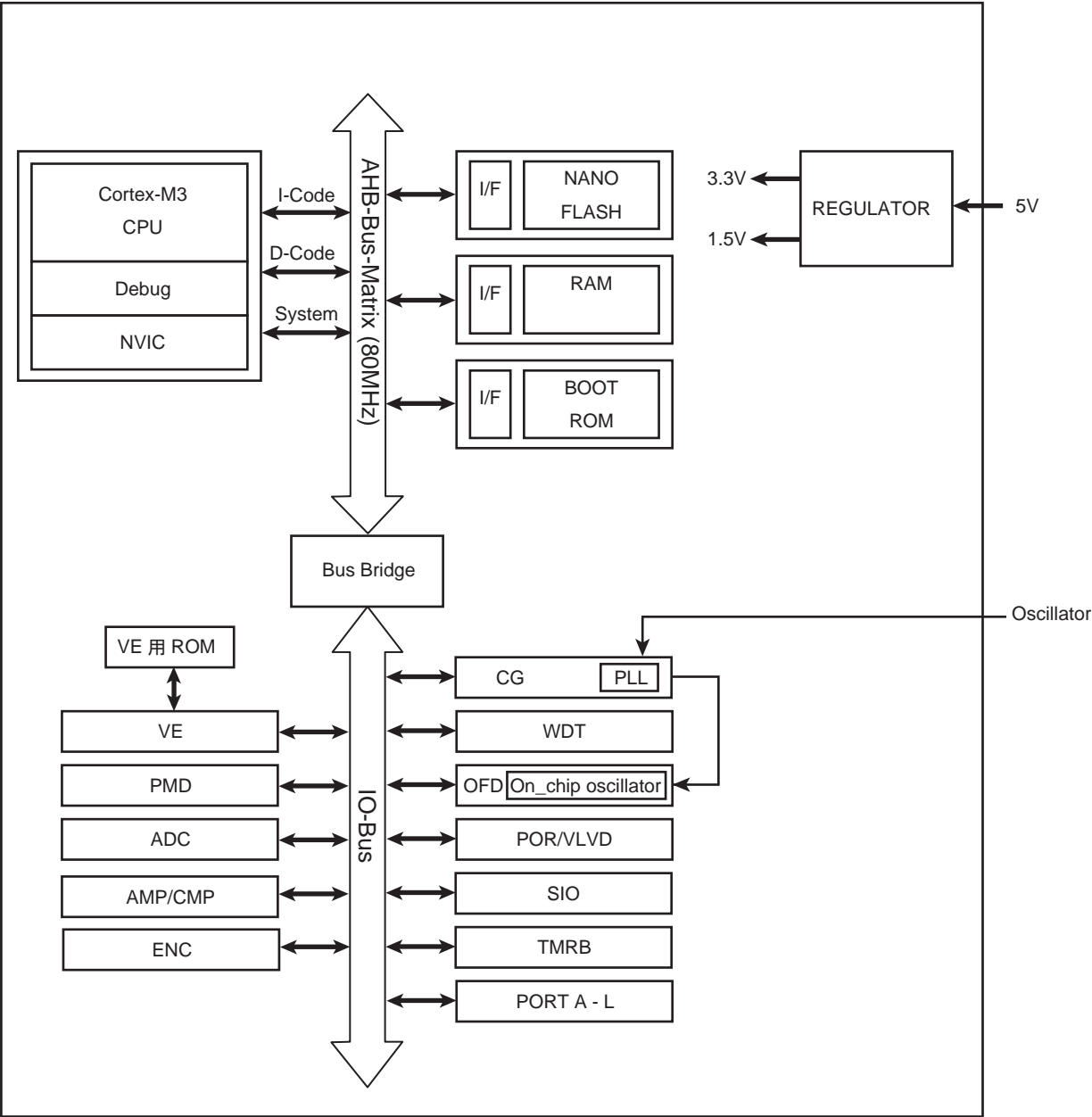
Figure 1-1 TMPM370FYDFG/FYFG block diagram
