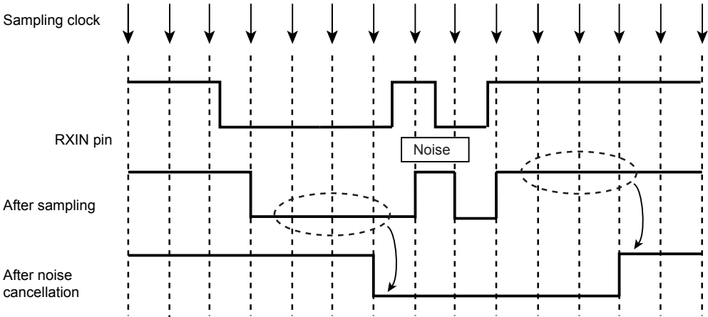
Figure 16-3 Noise Cancel (In the case of RMCRCR4="0011" (3 Cycles))
