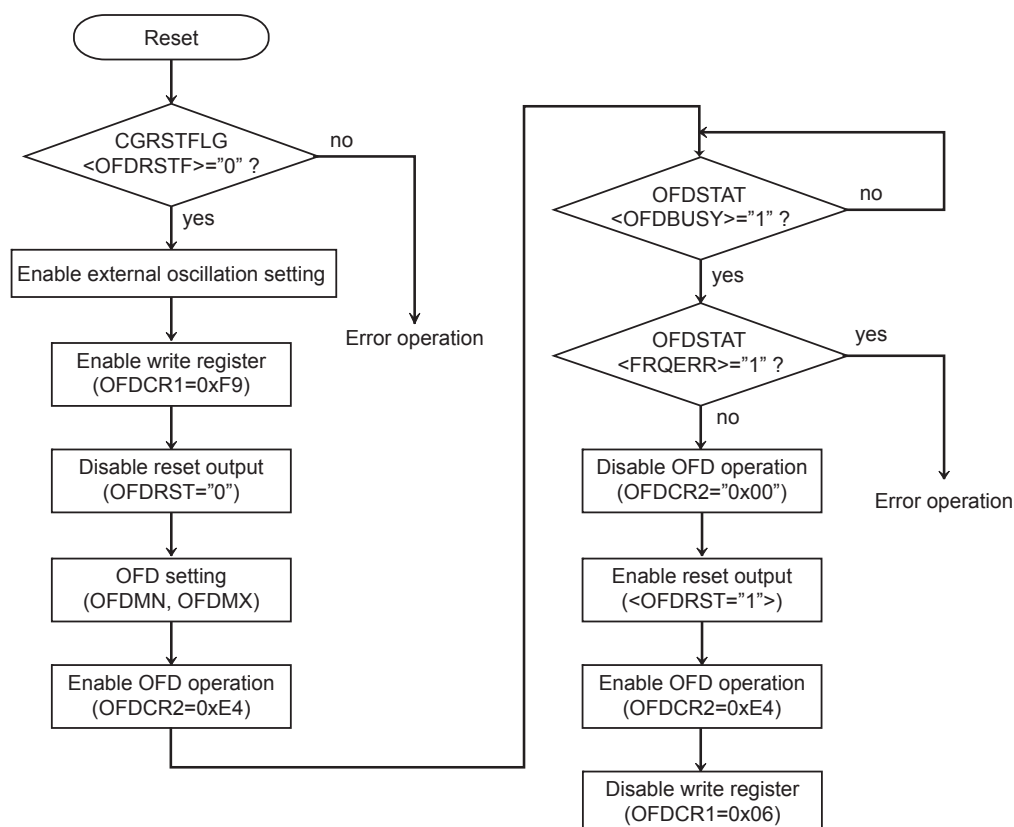
Figure 23-3 Example of operational procedure
