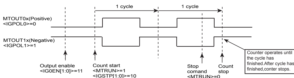
Figure 18-17 Counter stops with initial state after cycle has finished
