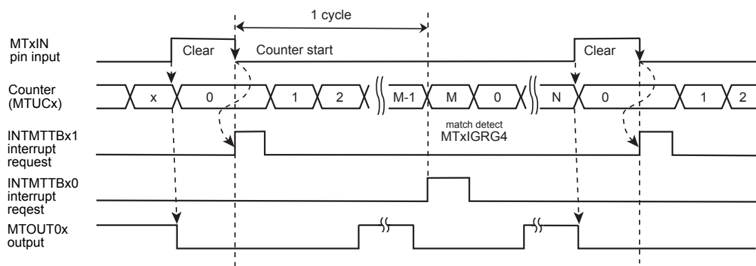
Figure 18-6 Trigger start interrupt operation
