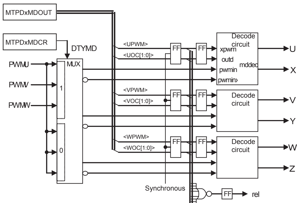
Figure 18-26 Schematic diagram of applying current control circuit
