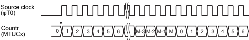
Figure 18-4 Count-up/clear operation when φT0 is selected as a source clock
