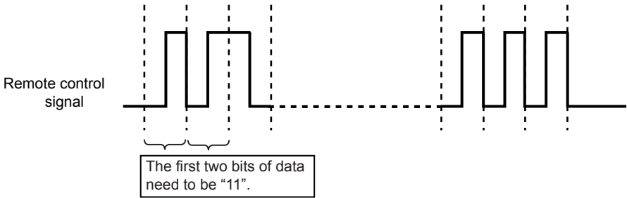
Figure 16-11 The waveform pattern in phase method
