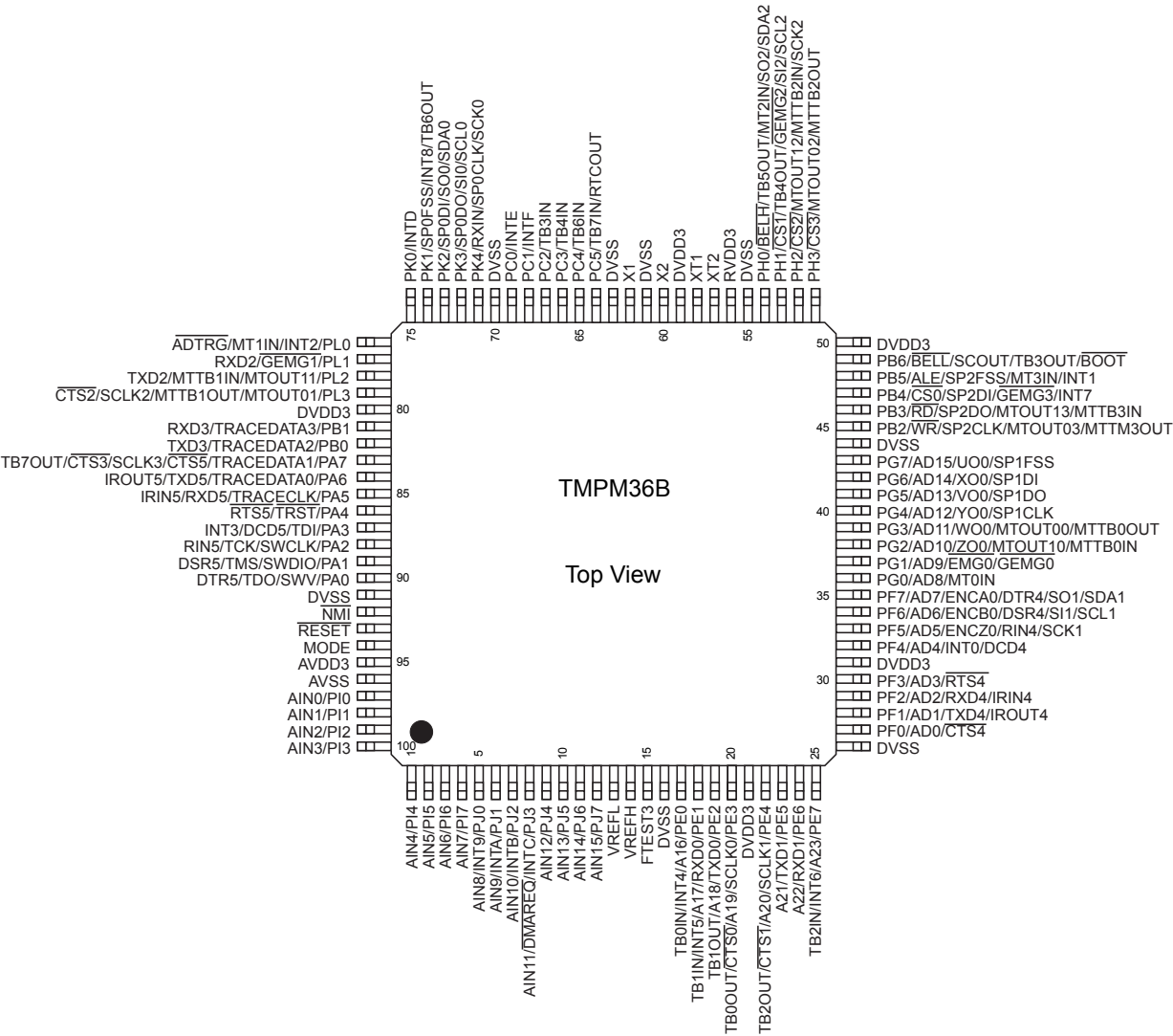
Figure 1-2 Pin Layout (LQFP100)
