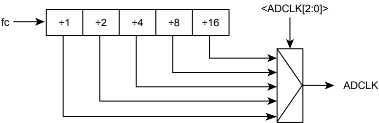
Figure 17-2 AD Conversion Clock (ADCLK)
