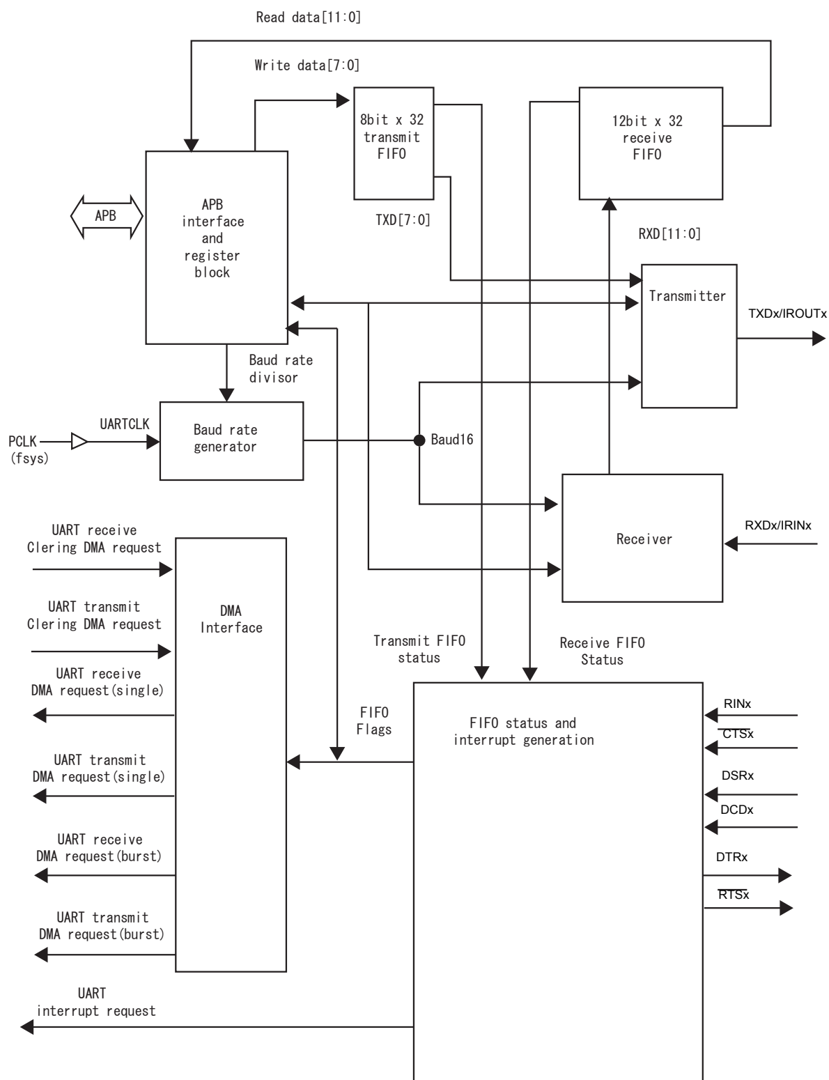
Figure 13-1 UART Channel Block Diagram
