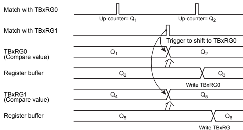
Figure 11-3 Register Buffer Operation
