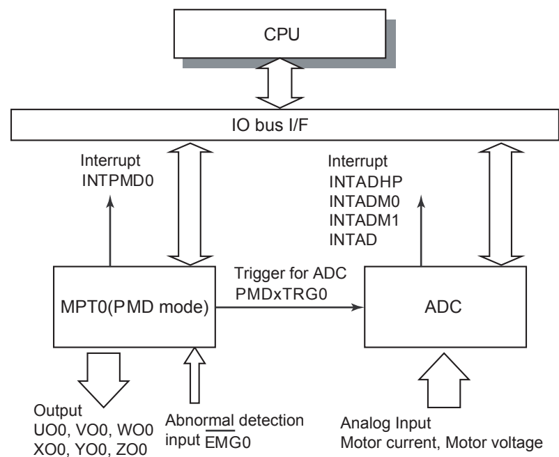
Figure 18-22 Block diagram of related with motor control
