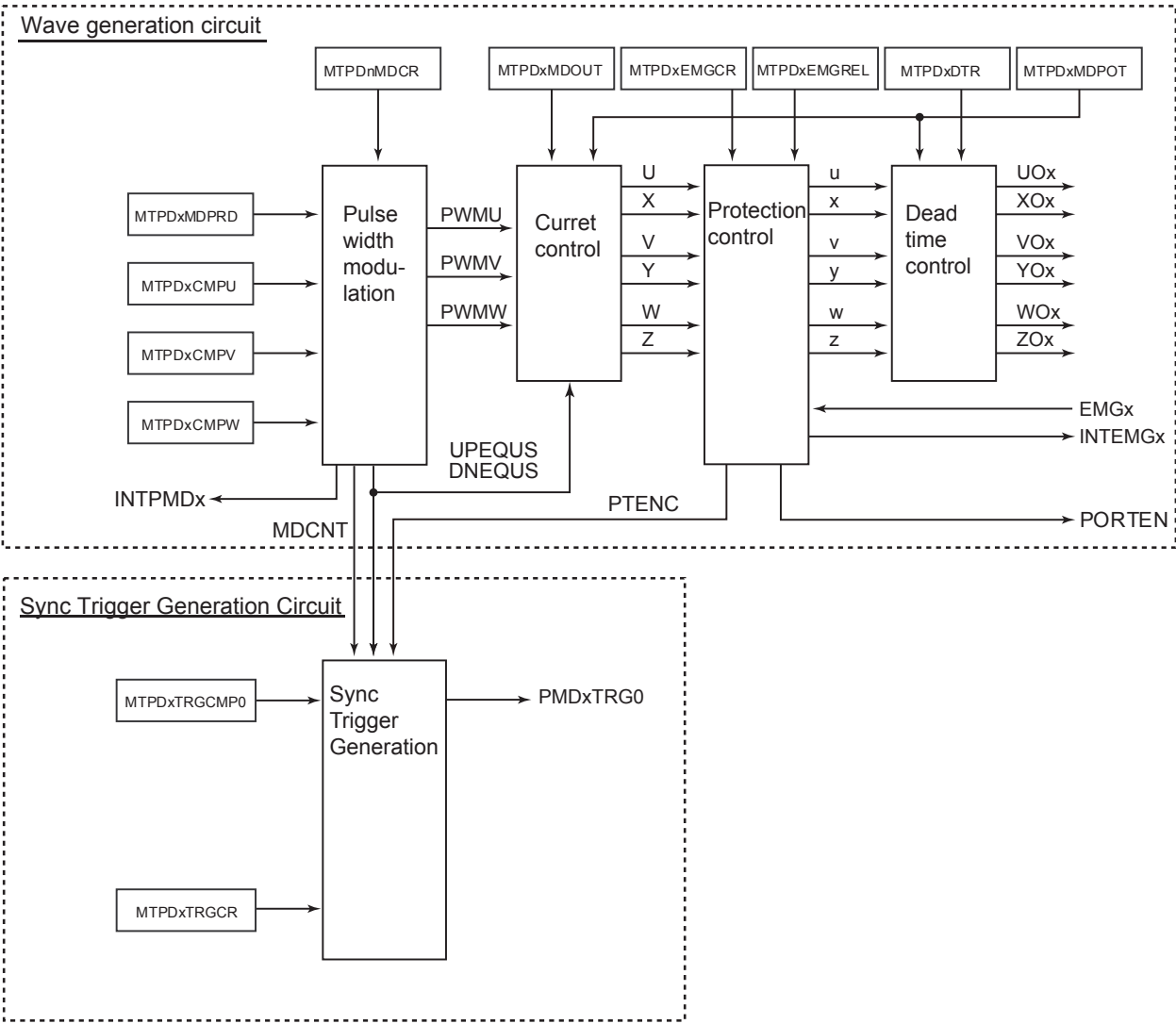
Figure 18-23 Schematic diagram of PMD circuit
