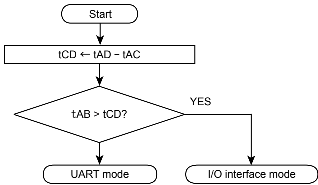
Figure 25-6 Serial Operation Mode Determination Flowchart
