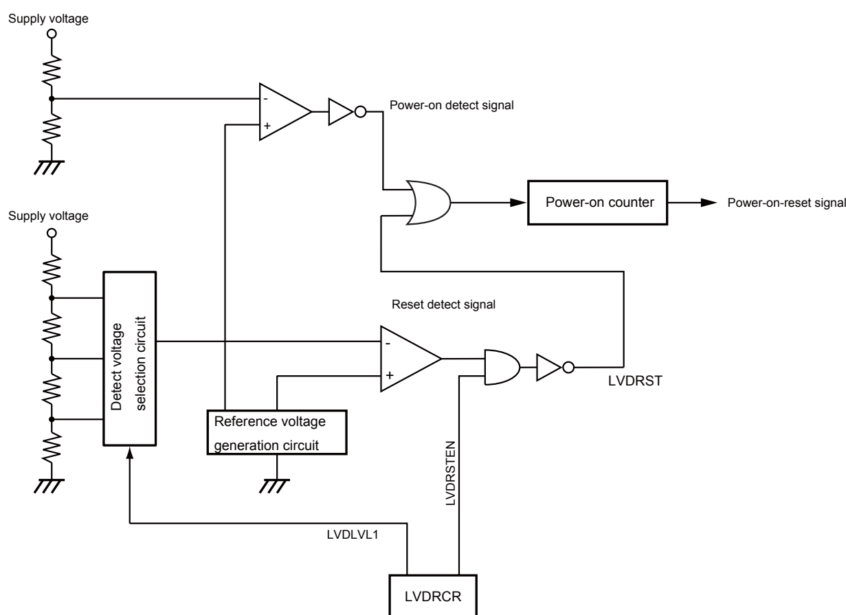
Figure 21-1 Power-on-reset circuit
