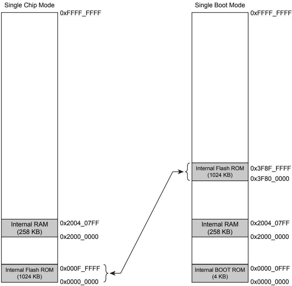
Figure 25-3 Memory Maps for TMPM36BF10FG
