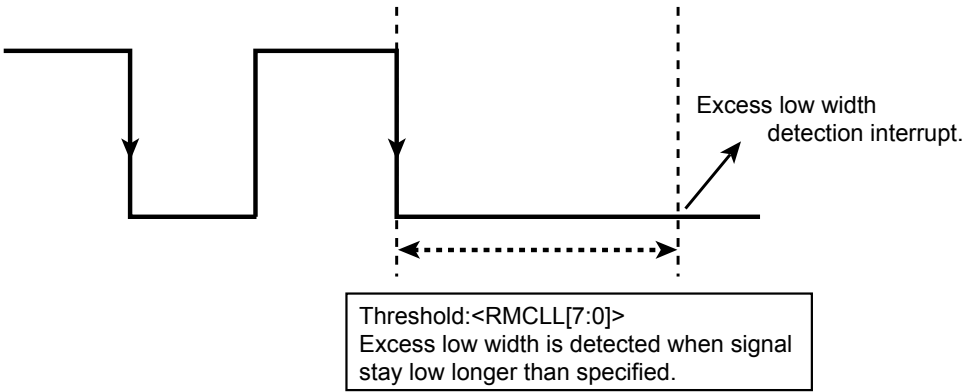
Figure 16-7 Completion by detecting low width
