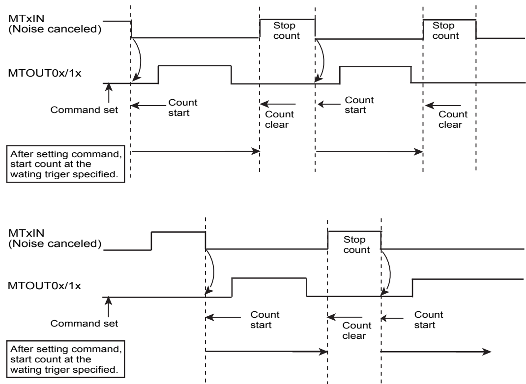
Figure 18-12 Trigger Start
