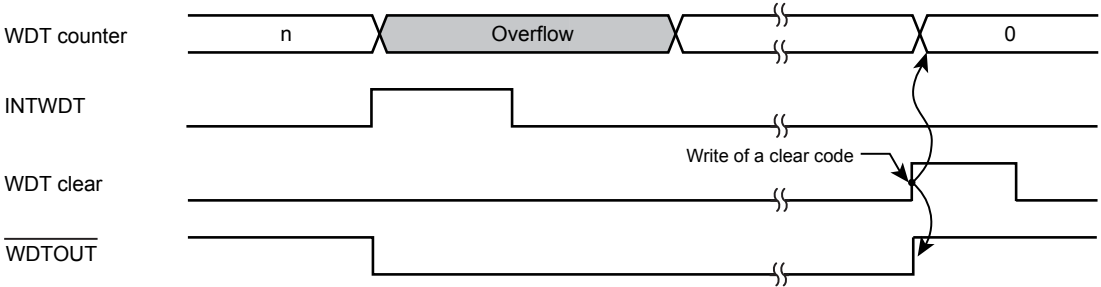
Figure 24-2 INTWDT interrupt generation
