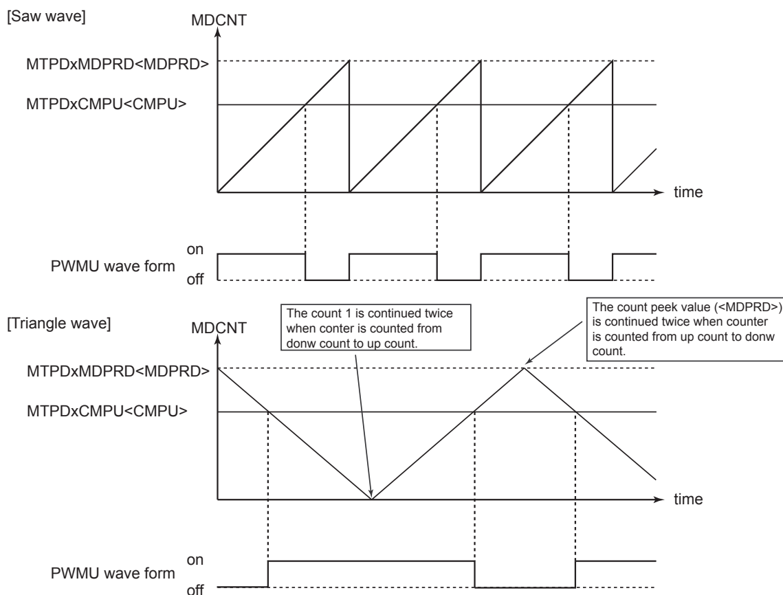
Figure 18-25 PWM waveform
