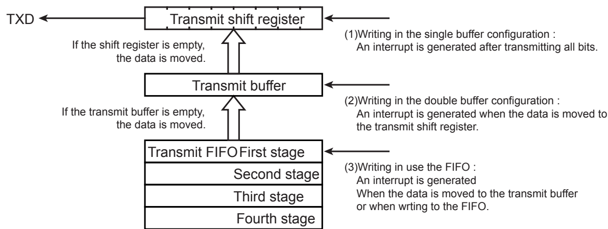
Figure 12-11 Transmit Buffer / FIFO Configuration Diagram
