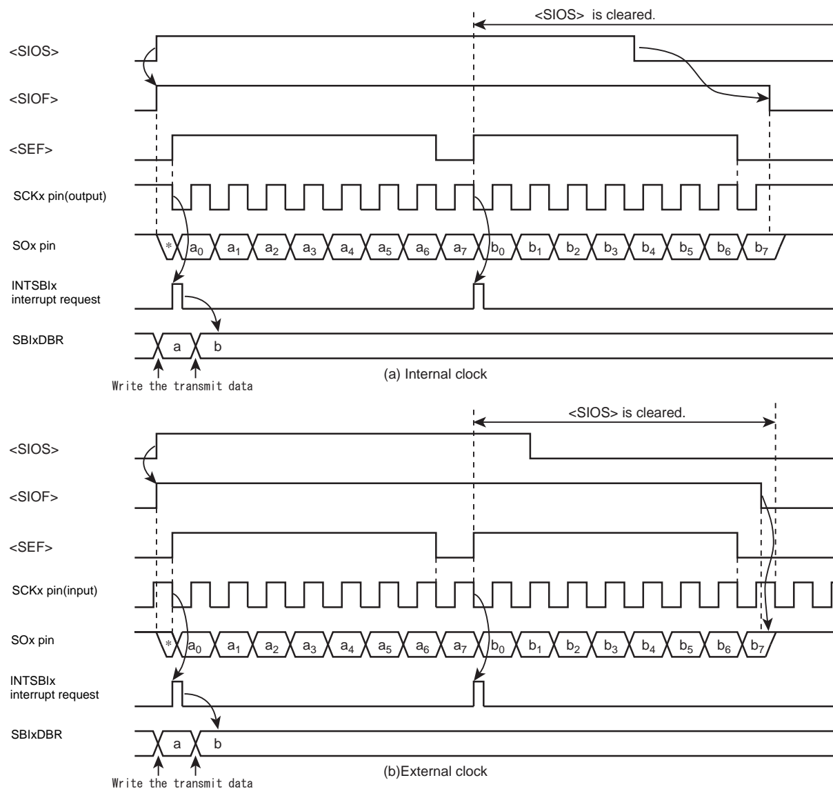
Figure 14-18 Transmit Mode
