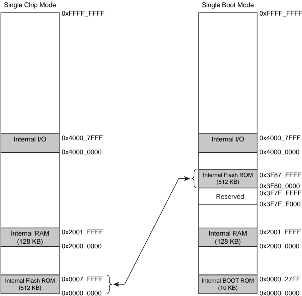
Figure 31-3 Memory Maps for TMPM369FDFG/XBG
