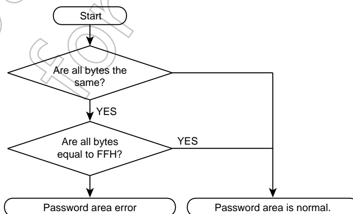
Figure 20-7 Password Area Verification Flowchart
