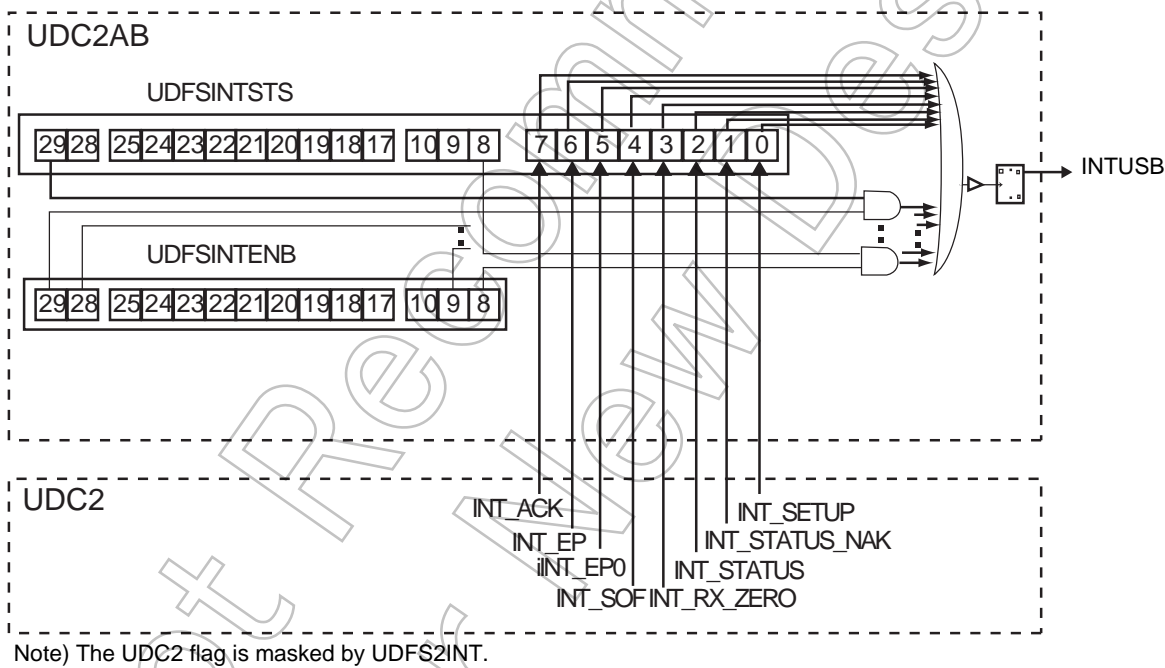
Figure 14-13 Relationship of INTUSB and registers
