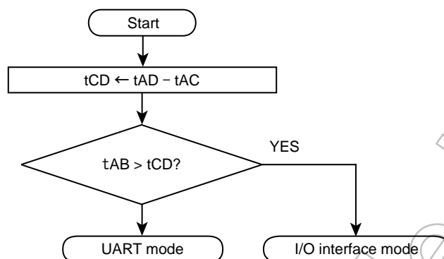
Figure 22-6 Serial Operation Mode Determination Flowchart
