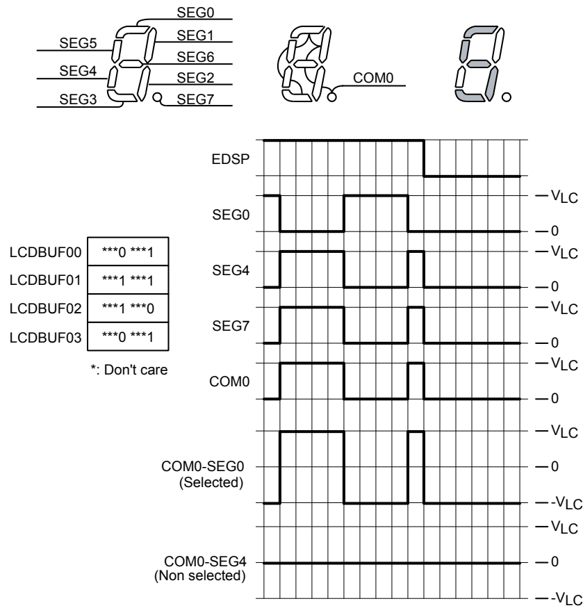
Figure 17-12 Static Drive
