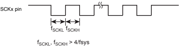
Figure 12-14 Maximum Transfer Frequency of External Clock Input
