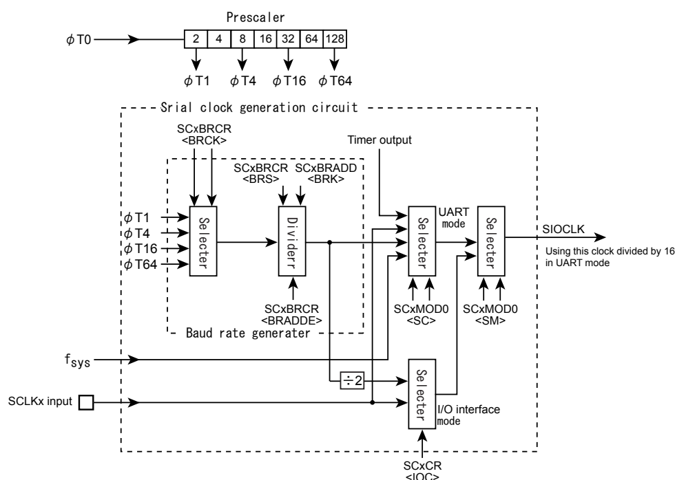
Figure 11-3 Serial clock generation circuit
