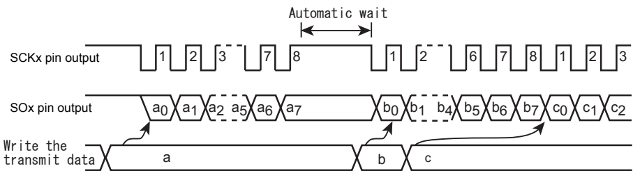
Figure 12-13 Automatic Wait
