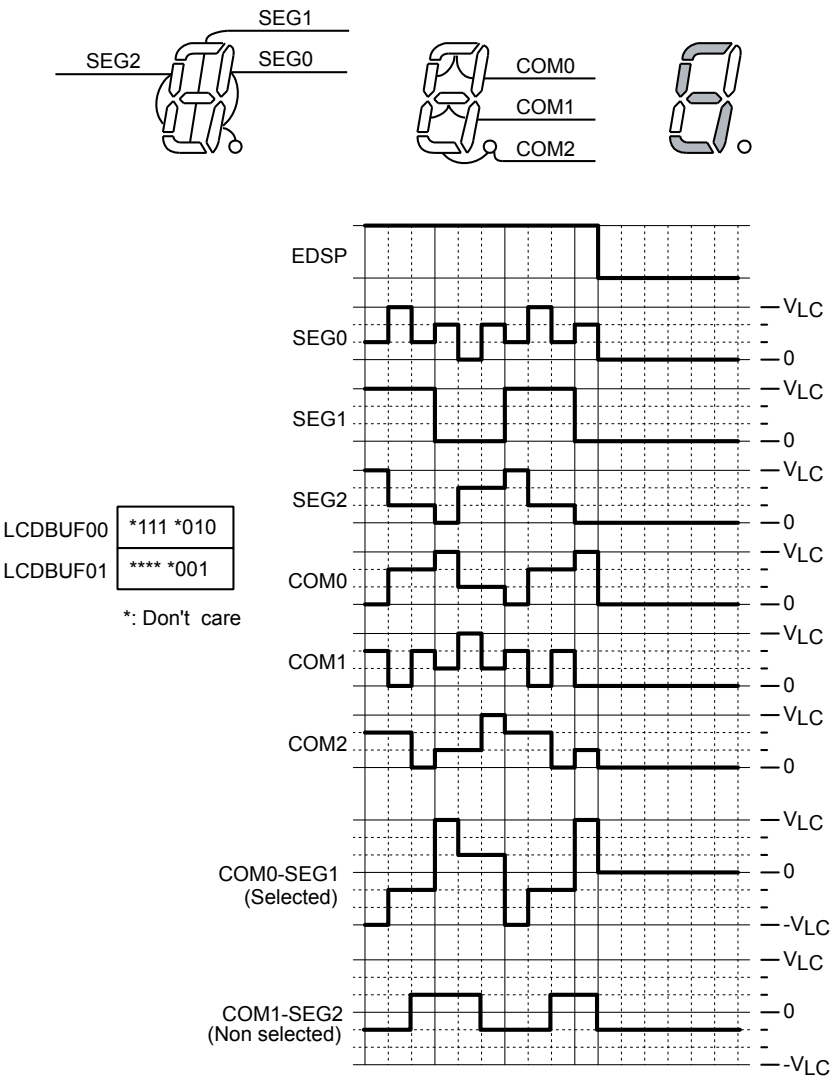
Figure 17-9 1/3 Duty (1/3 Bias) Drive
