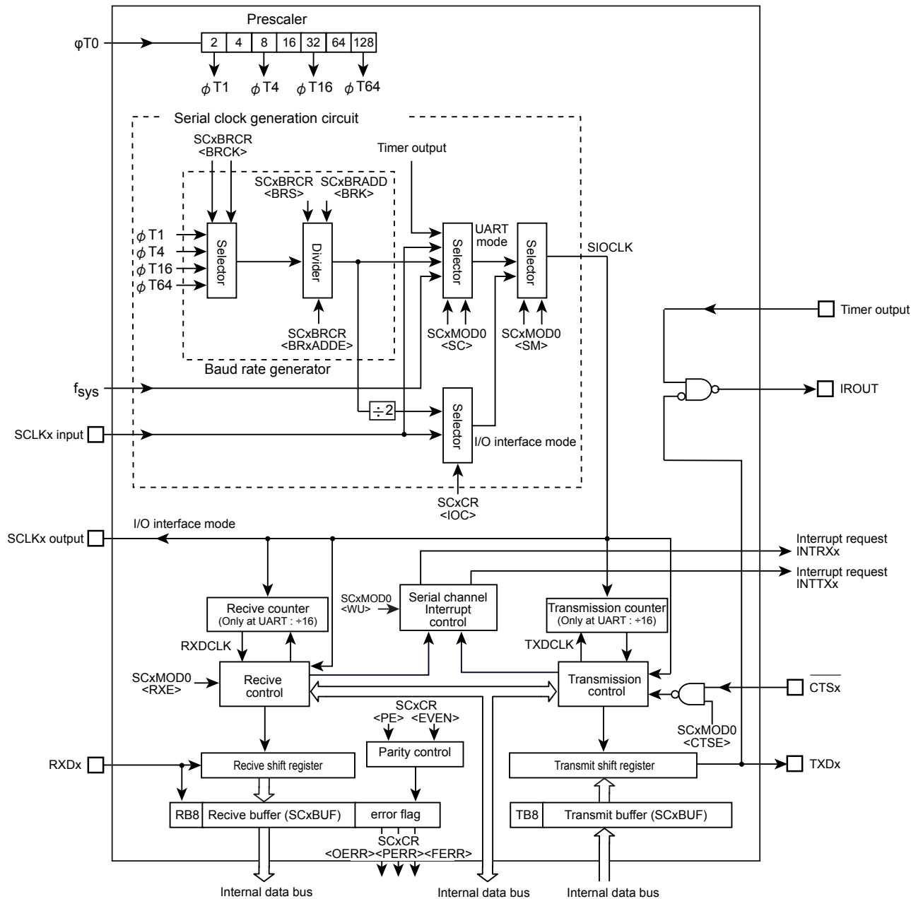
Figure 11-1 Serial Channel Block Diagram
