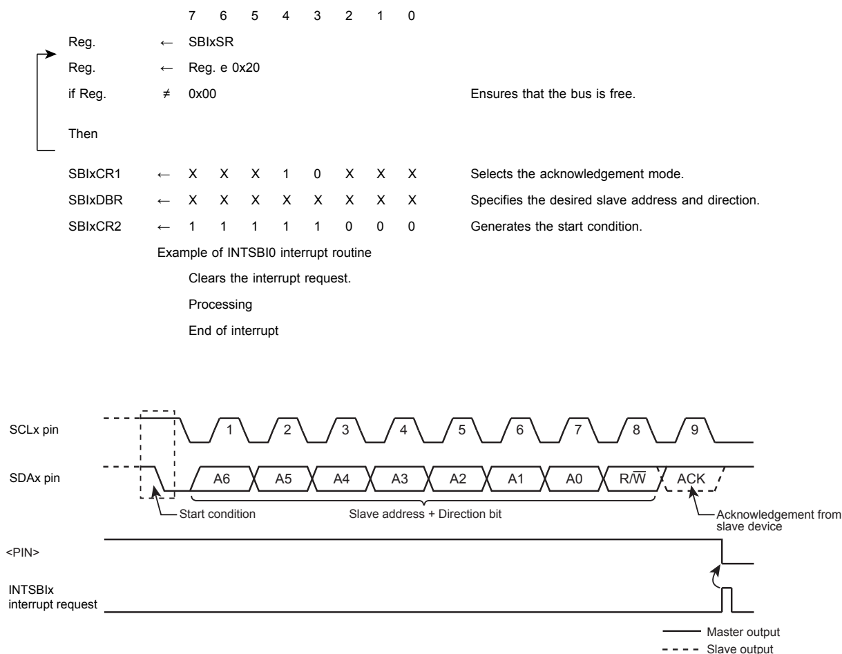
Figure 12-7 Generation of the Start Condition and a Slave Address
