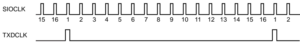
Figure 12-7 Generation of Transmission Clock in UART mode
