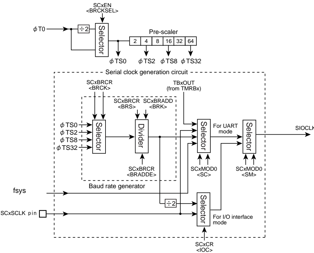
Figure 12-2 Serial clock generation circuit block diagram
