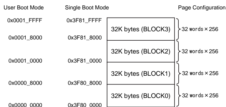
Figure 17-1 Block configuration
