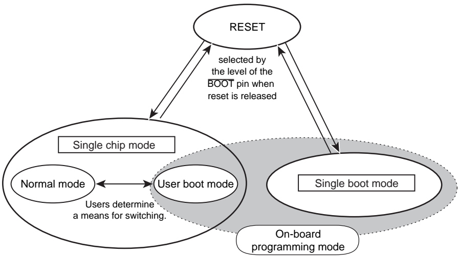
Figure 17-2 Mode transition
