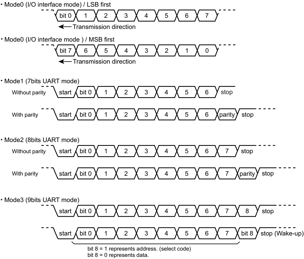
Figure 12-3 Data Format
