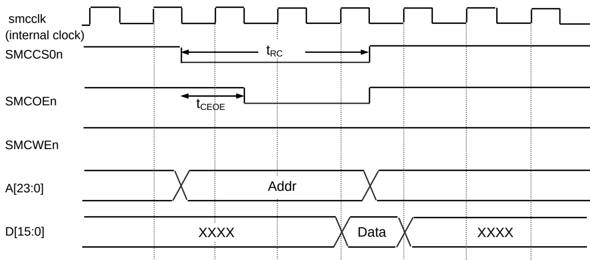
Figure 3.10.35 Asynchronous Read
