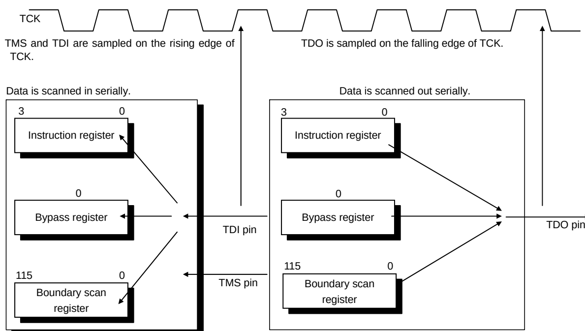
Figure 3.2.5 JTAG Test Access Port
