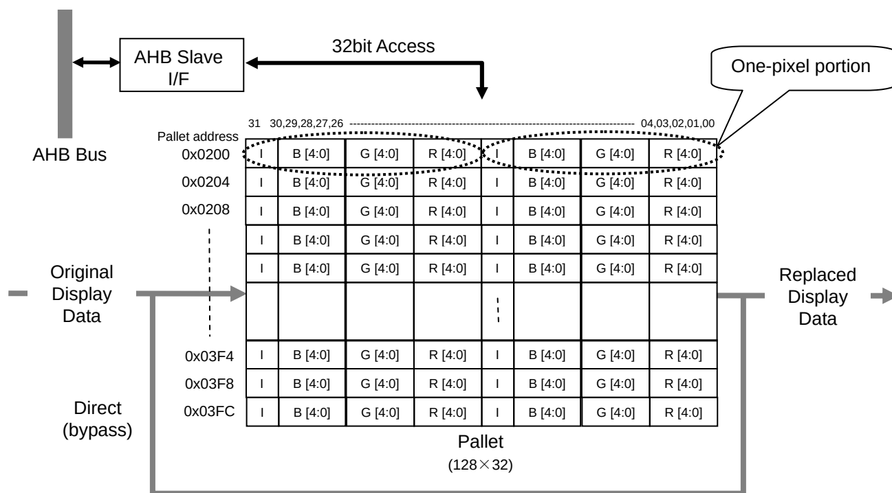
Figure 3.18.2 Palette RAM
