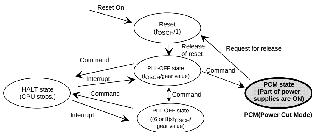
Figure 3.24.1 State Transition Diagram of TMPA901CM
