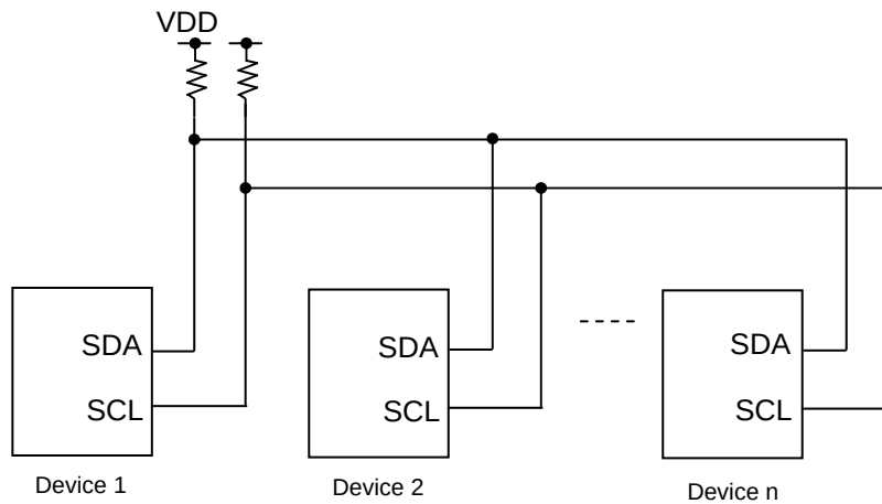
Figure 3.14.1 Device connections
