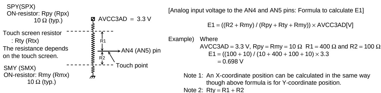
Figure3.20.5 Analog input voltage calculation values
