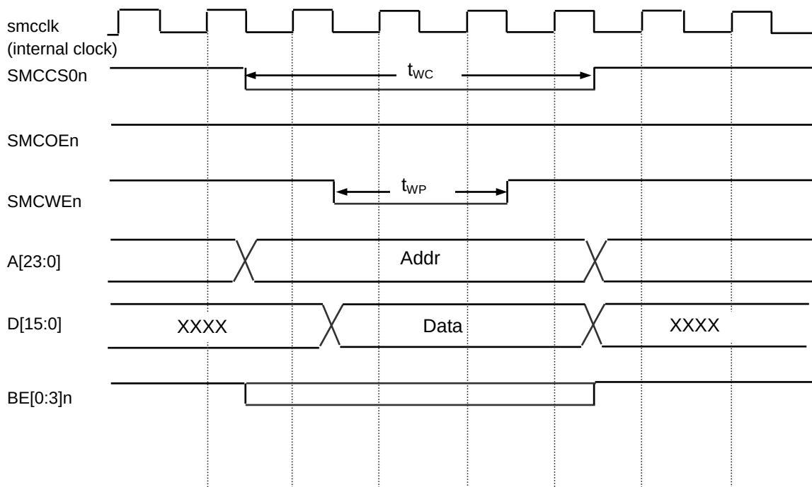
Figure 3.10.36 Asynchronous Write
