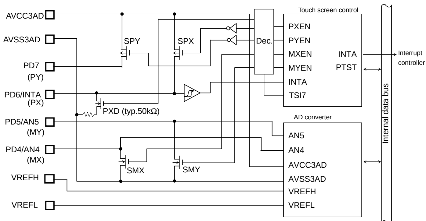
Figure 3.20.2 Internal block diagram of TSI
