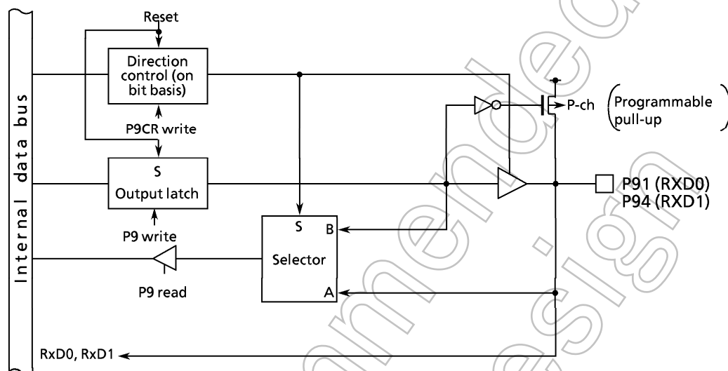
Figure3.5 (18) Ports 91 and 94
