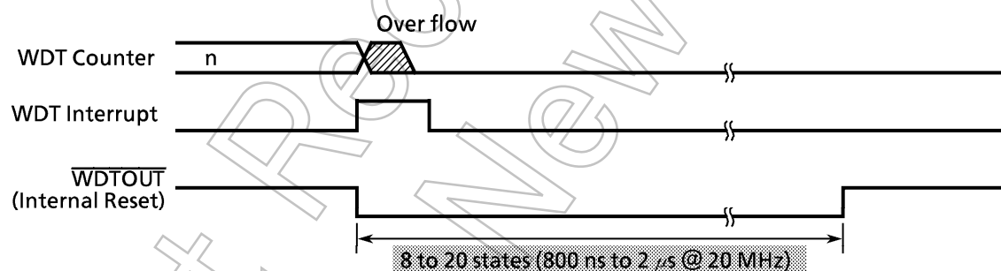
Figure 3.13 (3) Reset Mode
