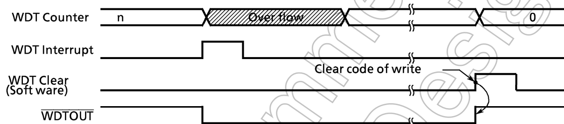
Figure 3.13 (2) Normal Mode
