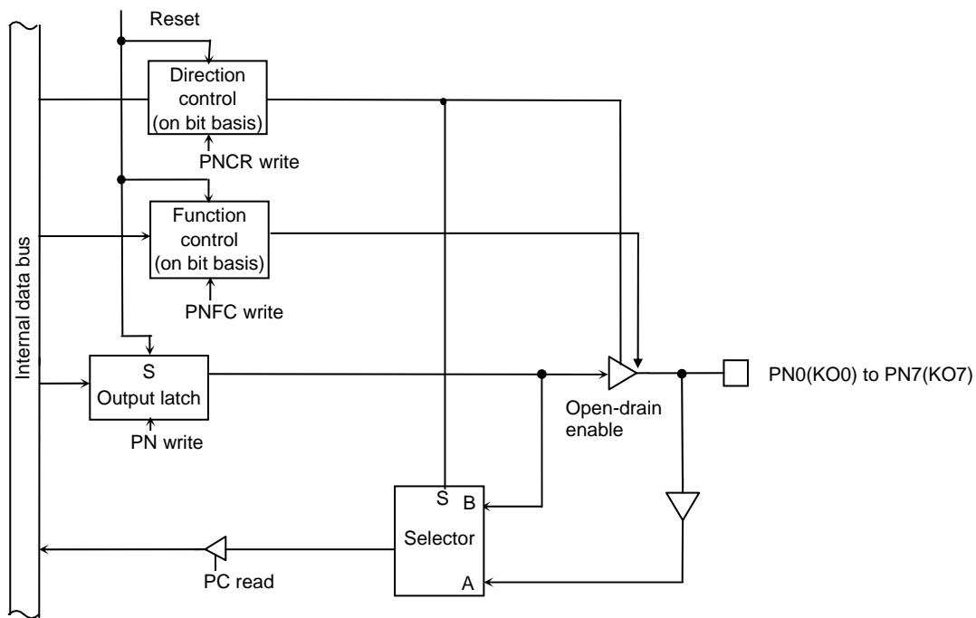
Figure 3.7.42 Port N
