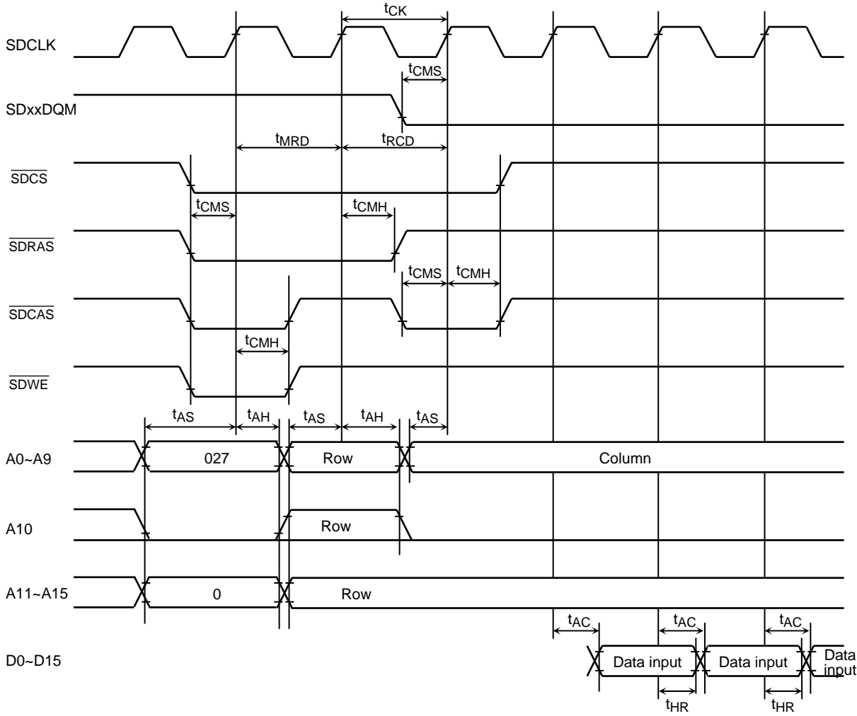
(3) SDRAM burst read timing (Start burst cycle)
