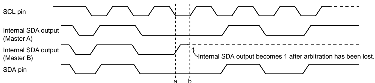
Figure 3.15.12 Arbitration lost
