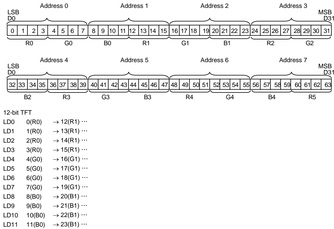
Figure 3.19.9 Memory Map Image and Data Output in TFT 4096-Color Mode
