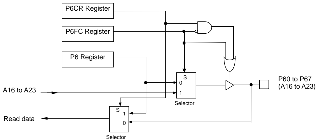
Figure 3.7.7 Port6
