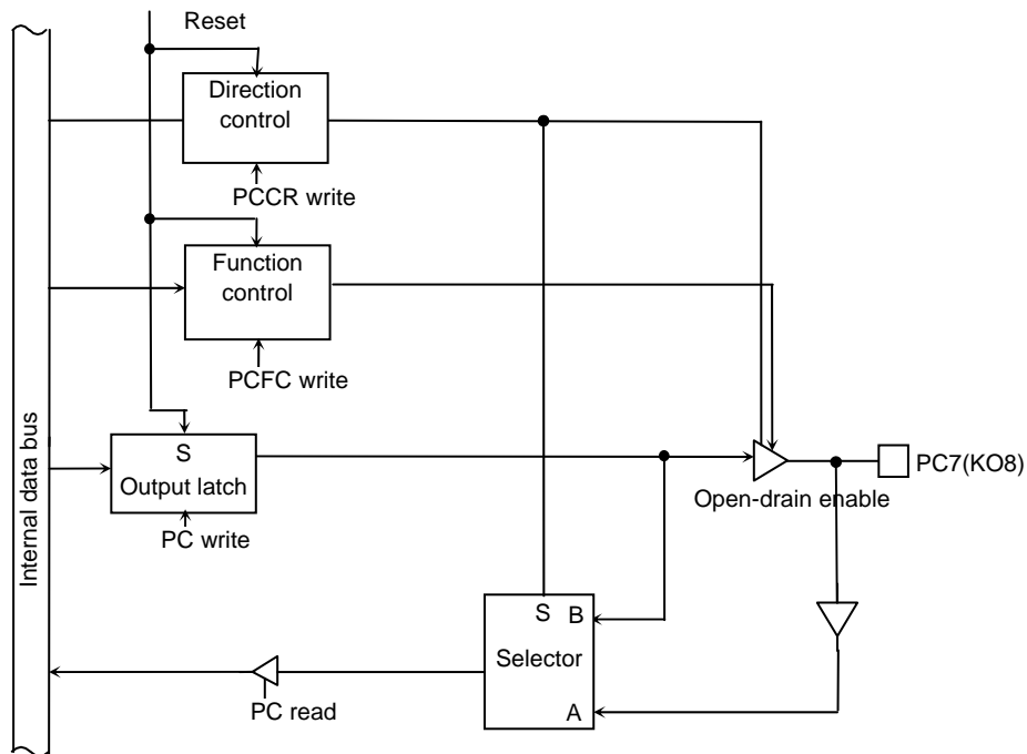
Figure 3.7.23 Port C7
