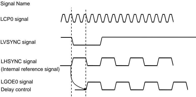
LGOE0 Delay Register
