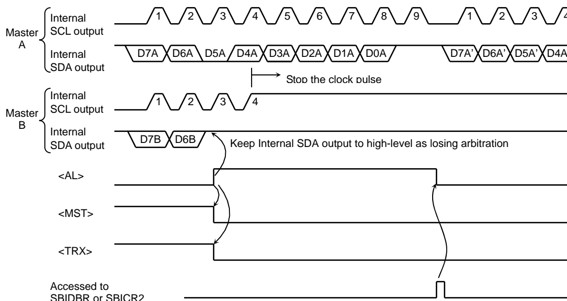
Figure 3.15.13 Example of when TMP92CZ26A is a master device B
