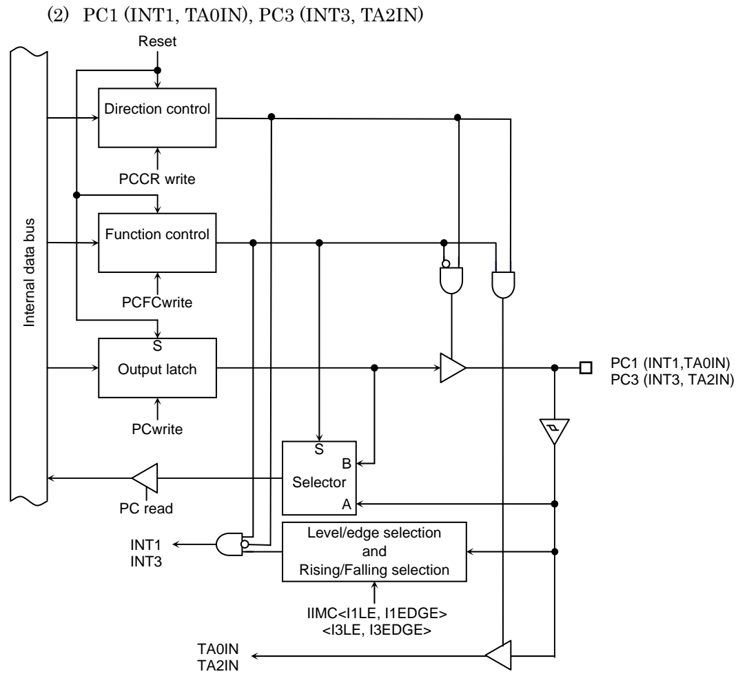
Figure 3.7.21 Port C1, C3
