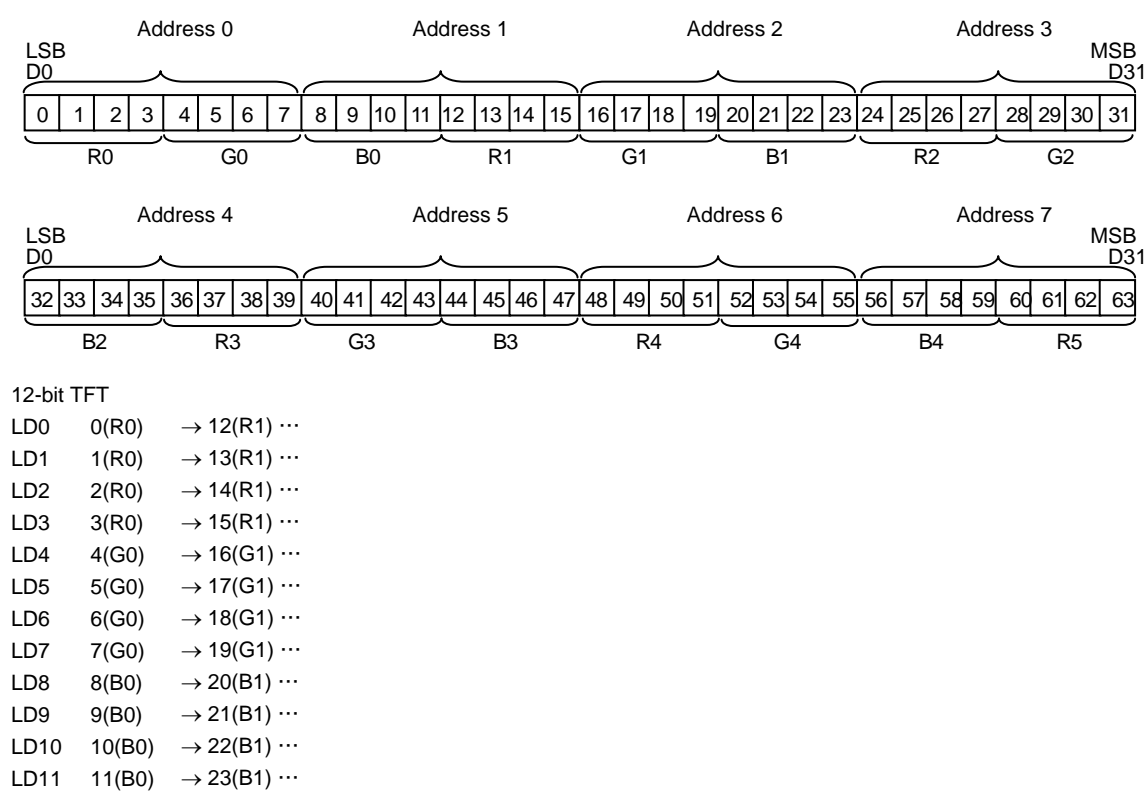
Figure 3.20.10 Memory Map Image and Data Output in TFT 4096-Color Mode
