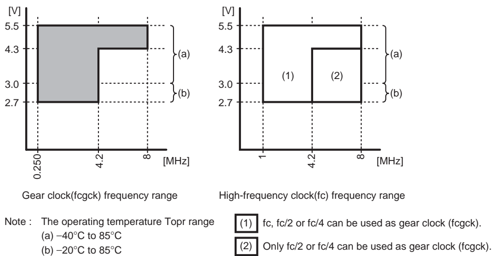
Figure 25-2 Clock gear (fcgck) and High-frequency clock (fc)
