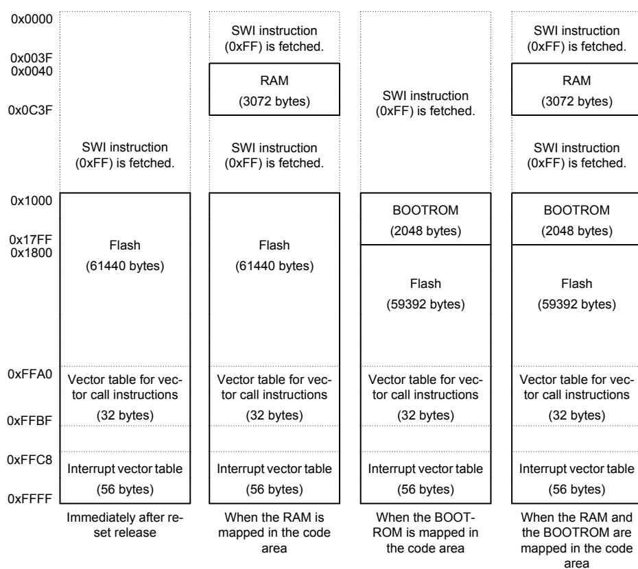
Figure 2-1 Memory Map in the Code Area
