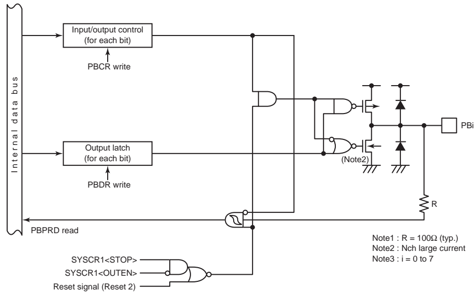
Figure 8-11 Port PB
