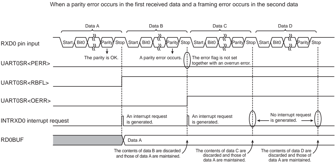
Figure 16-13 Framing/Parity Error Flags When an Overrun Error Occurs
