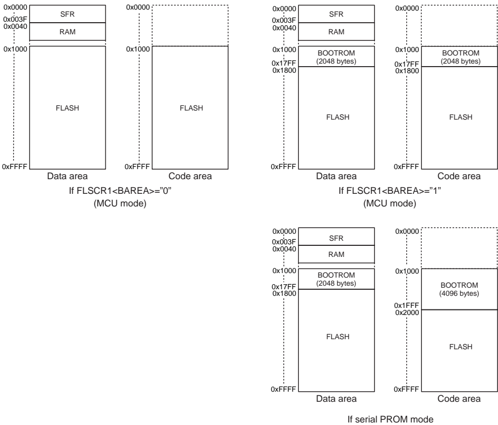
Figure 22-3 Memory Mapping
