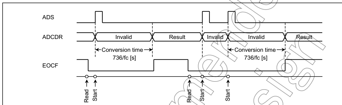
Figure 2.12.4 AD Conversion Timing Chart (ACK = 1)
