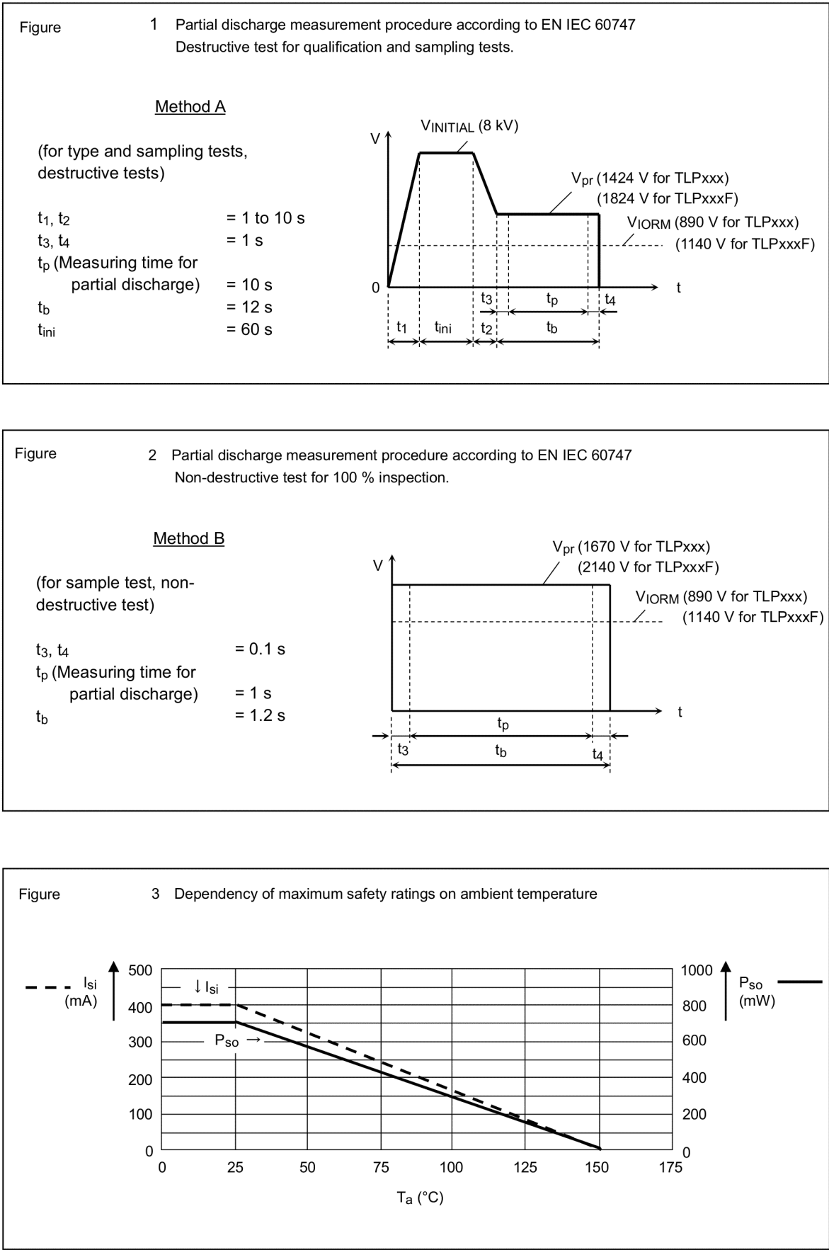
Fig. 16.5 Measurement Procedure
