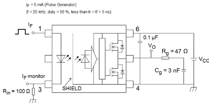
Fig. 13.1.6 Switching Time Test Circuit and Waveform
