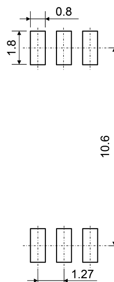
Fig. 15.2 Lead Forming Option (LF4)
