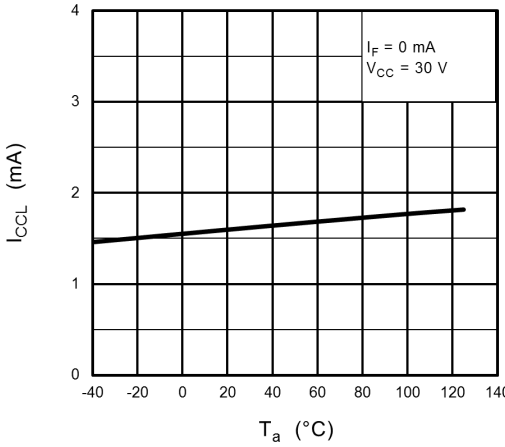
Fig. 13.2.5 I_{CCL} - T_a
