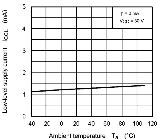
Fig. 13.2.5 I_{CCL} - T_a
