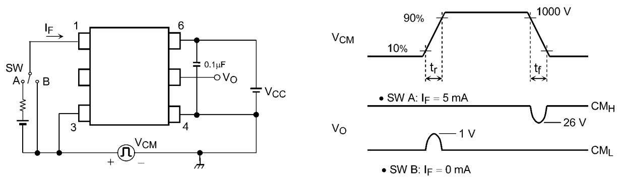
Fig. 13.1.8 Common-Mode Transient Immunity Test Circuit and Waveform
