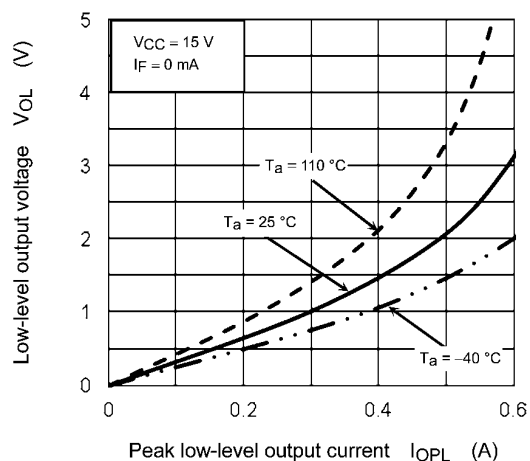
Fig. 13.2.9 V_{OL} - I_{OPL}
