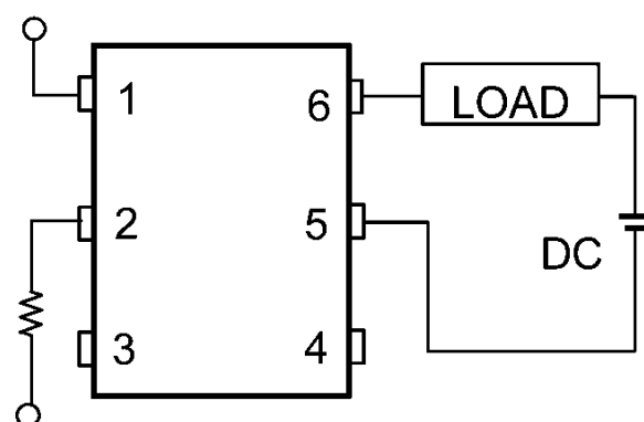
Fig. 14.2 B connection
