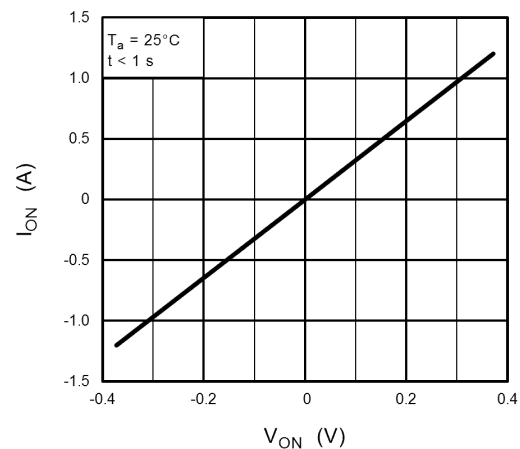
Fig. 14.4 I_{\text{ON}} - V_{\text{ON}}
