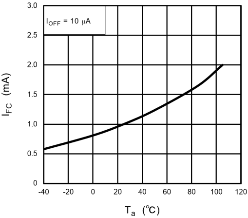
Fig. 12.6 I_{FC} - T_a
