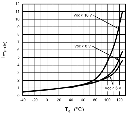
Fig. 12.4 I_{FT}(\text{ratio}) - T_a
