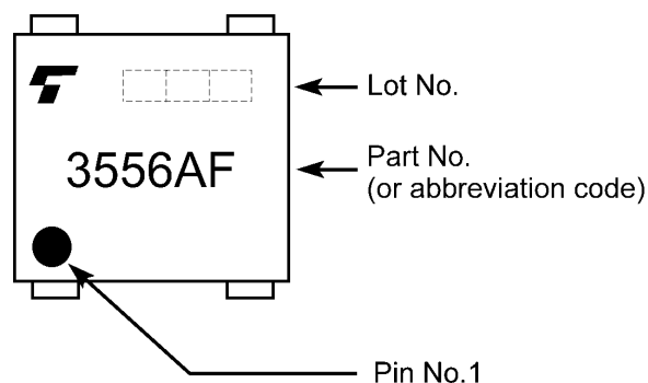
TLP3556AF
