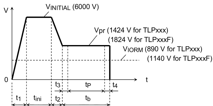
Figure 2 Partial discharge measurement procedure according to EN 60747 Non-destructive test for 100% inspection.
