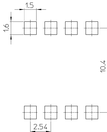
Fig. 18.2 Lead forming and taping option (LF4), (TP4)
