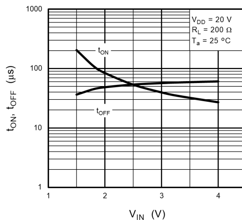
Fig. 12.6 t_{ON}, t_{OFF} - V_{IN}
