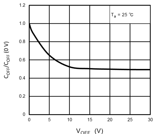
Fig. 12.11 C_{OFF}/C_{OFF} - V_{OFF}
