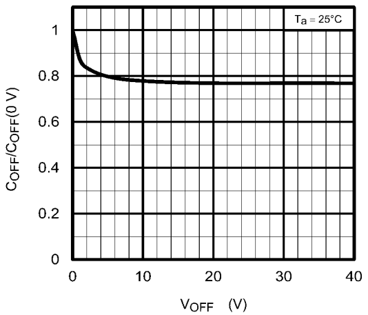
Fig. 12.1.11 C_{OFF}/C_{OFF(0V)} - V_{OFF}
