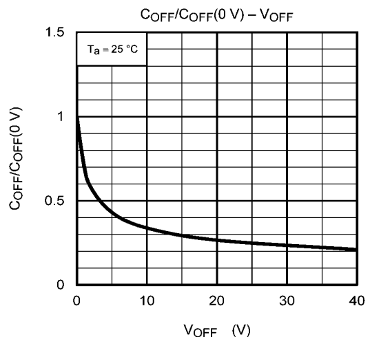
Fig. 12.1.11 C_{OFF}/C_{OFF}(0\text{ V}) - V_{OFF}
