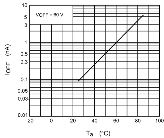
Fig. 12.9 IOFF - Ta
