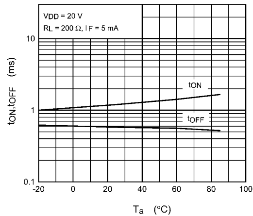
Fig. 12.7 tON,tOFF - Ta
