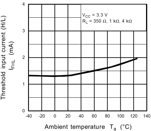
Fig. 13.2.8 I_{FHL} - T_a
