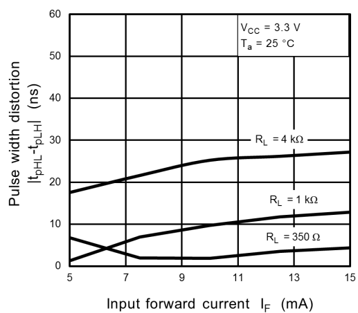
Fig. 13.2.24 |t_{pHL} - t_{pLH}| - I_F
