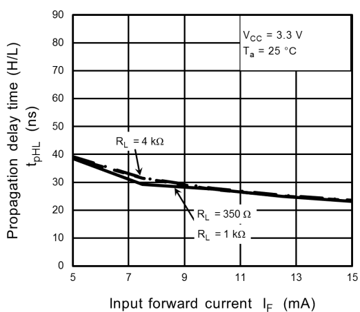
Fig. 13.2.22 t_{pHL} - I_F
