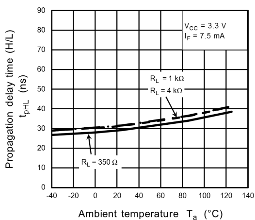
Fig. 13.2.16 t_{pHL} - T_a
