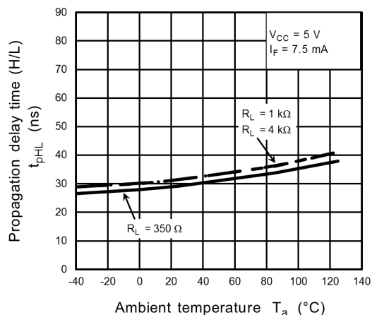
Fig. 13.2.13 t_{pHL} - T_a
