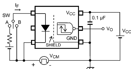
Fig. 14.1.6 Common-Mode Transient Immunity Test Circuit and Waveform
