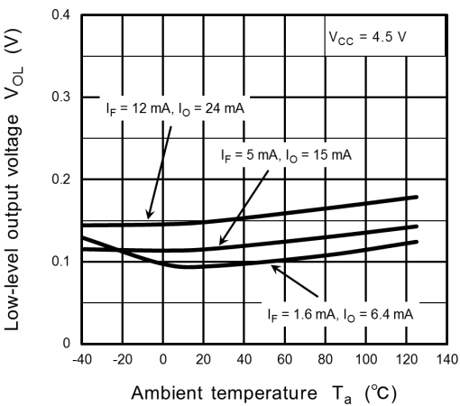
Fig. 12.2.6 V_{OL} - T_a
