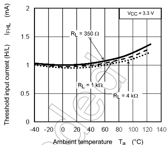
Fig. 12.2.8 I_{FHL} - T_a
