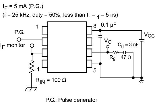
Fig. 12.1.7 Switching Time Test Circuit and Waveform
